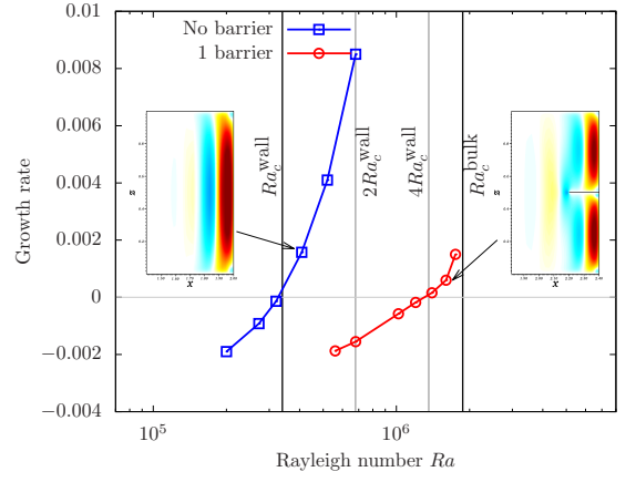
FIG. 4. Growth rate as a function of Ra for E = 10^{-4} for the reference case with no barrier and the case with one barrier of width \epsilon = 0.2 located at z = 1/2 . The insets show the vertical component of the velocity in the y = 0 plane during the exponential growth phase.
