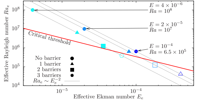
FIG. 5. Effective Rayleigh number Ra_e versus the effective Ekman number E_e . The symbols indicate the number of barriers starting from N = 0 where Ra_e = Ra and E_e = E . Filled (empty) symbols indicate growing (decaying) wall modes. The thick red line is the critical curve for the onset of wall modes predicted by linear theory [33] while the thin grey lines show the Ra_e \sim E_e^{-2} scaling.
