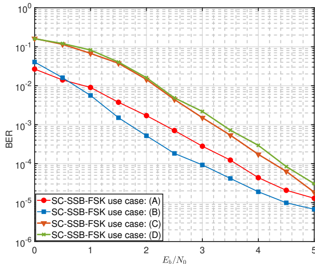
FIGURE 12. BER plots for the use case (A, B, C, and D).
