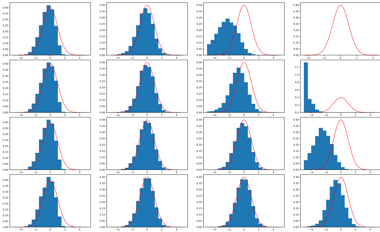
FIGURE 9. Empirical distribution of standardized \hat{\mathcal{F}}_n^m for r = 0.3 . The value of m increases from 10^5 on the top row up to 10^8 in the bottom row. The value of n increases from 10^1 on the left column up to 10^4 in the right column.
