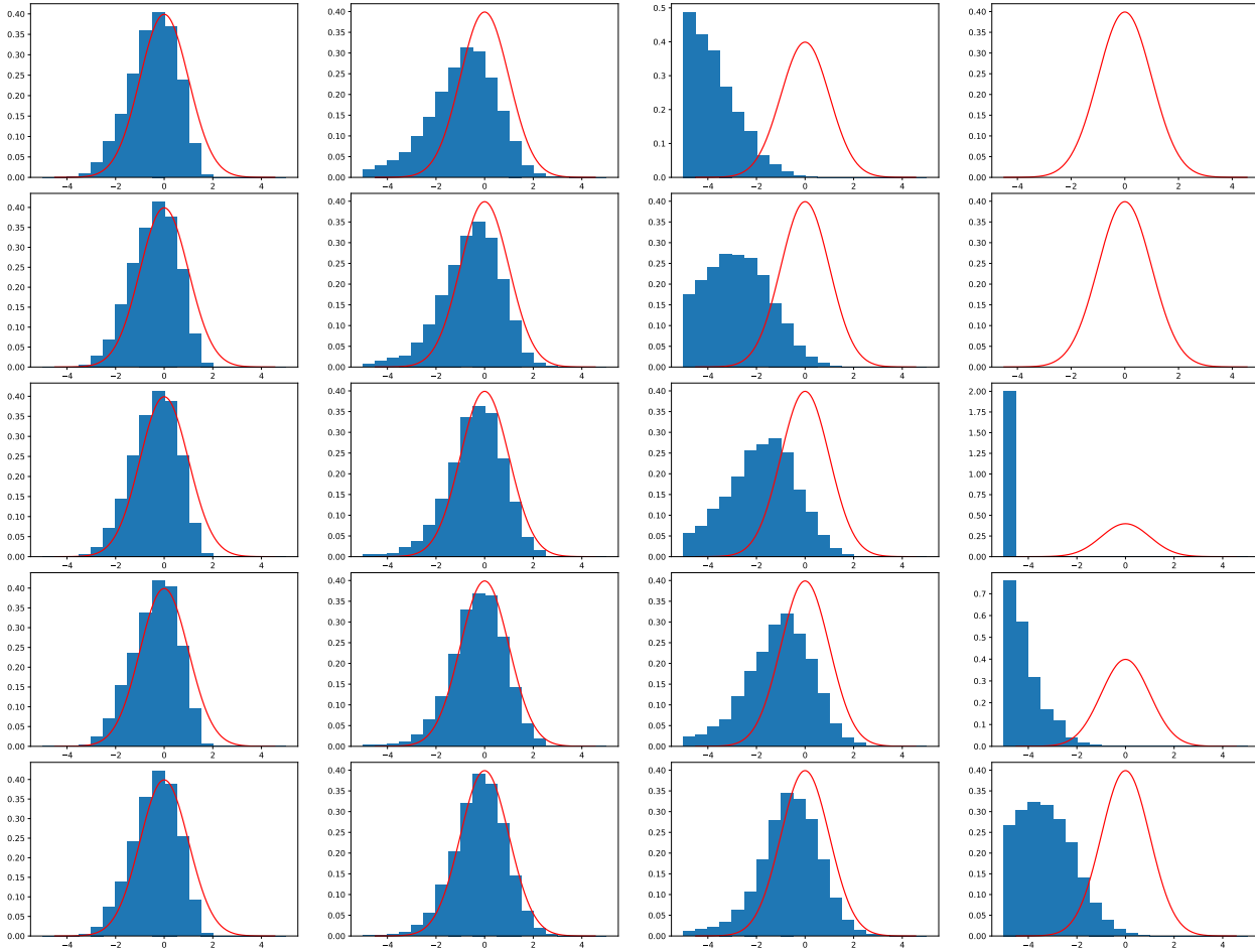
FIGURE 10. Empirical distribution of standardized \widehat{\mathcal{F}}_n^m for r = 0.4 . The value of m increases from 10^5 on the top row up to 10^9 in the bottom row. The value of n increases from 10^1 on the left column up to 10^4 in the right column.
