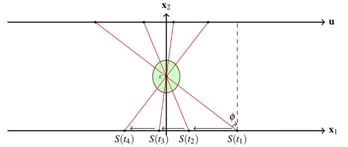
Figure 2: The equivalent radiography system. The source and the detector are moving at the same speed in the opposite direction to the translation of the conveyor belt in the Fig. 1. The object is stationary.
