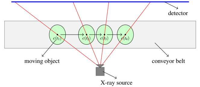
Figure 1: The radiography system is constituted of a X-ray source, a horizontal linear detector and a conveyor belt. Everything is stationary, except for the object translating on the conveyor belt.
