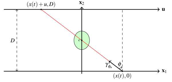
Figure 3: The parallel linogram. The object is supposed stationary and its center of mass is denoted by c . For a viewing angle \phi , the offset u = D \tan \phi between the source and the projection point on the detector is constant. The position of the source and the projection point associated to \phi are respectively (x(t), 0) and (x(t) + u, D) .
