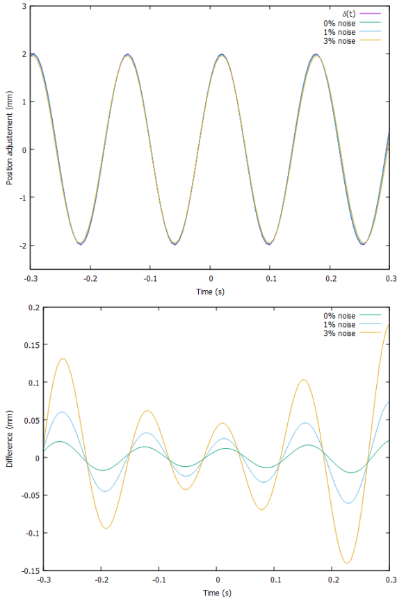
Figure 4: Estimation of the motion variation \delta(t) = A \sin(\omega t + \psi) with 0%, 1% and 3% Gaussian noise. Top: the function \delta(t) and its estimates. Bottom: difference between the theoretical value of \delta(t) and its estimates.
