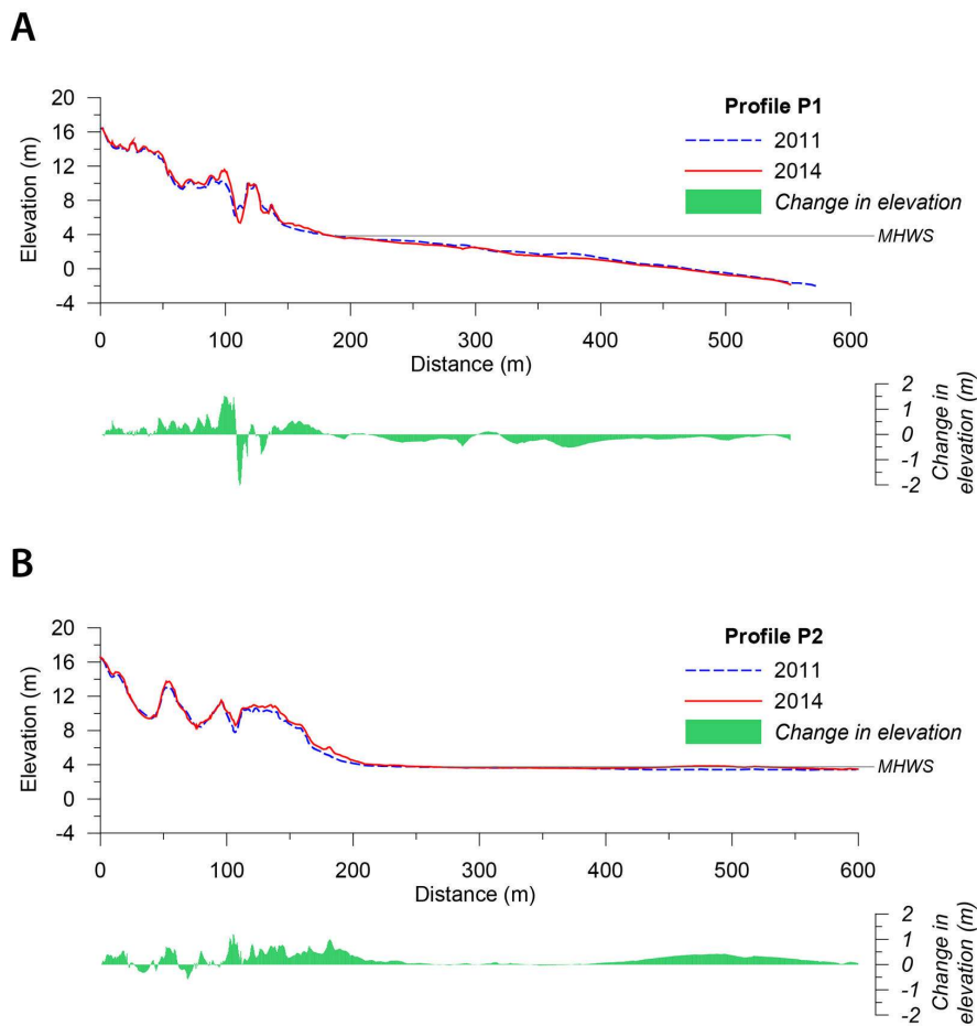
Fig. 9 – Cross-shore DGPS topographic profiles of the beach and coastal dunes east of Calais.
