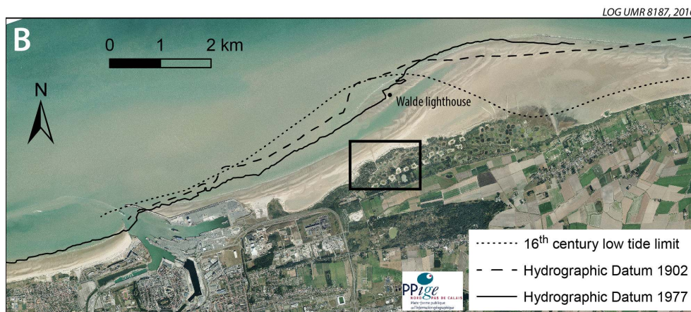
Fig. 3 – Changes in the position of tide levels since the 16 th century.
