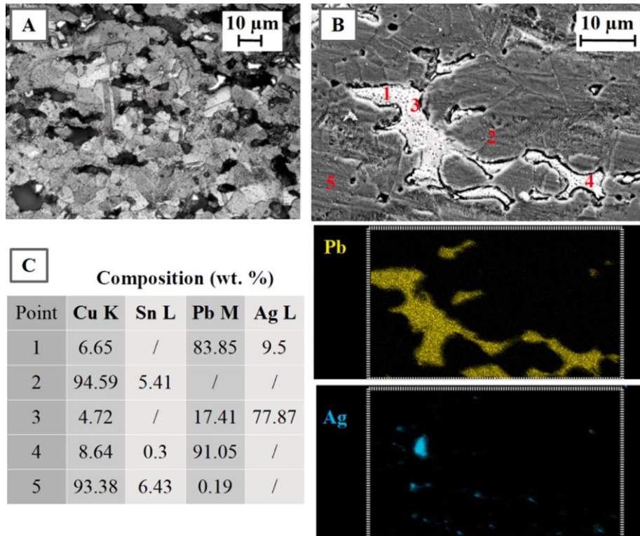
Fig. 4. Coin 2: microstructure of coin's bulk after etching in aqueous \text{FeCl}_3 solution. OM-Leica image (A); FESEM-Supra-secondary electron image and correspondent maps of the Pb and Ag elements (B); indication of the EDS punctual analyses with corresponding EDS composition (C).
