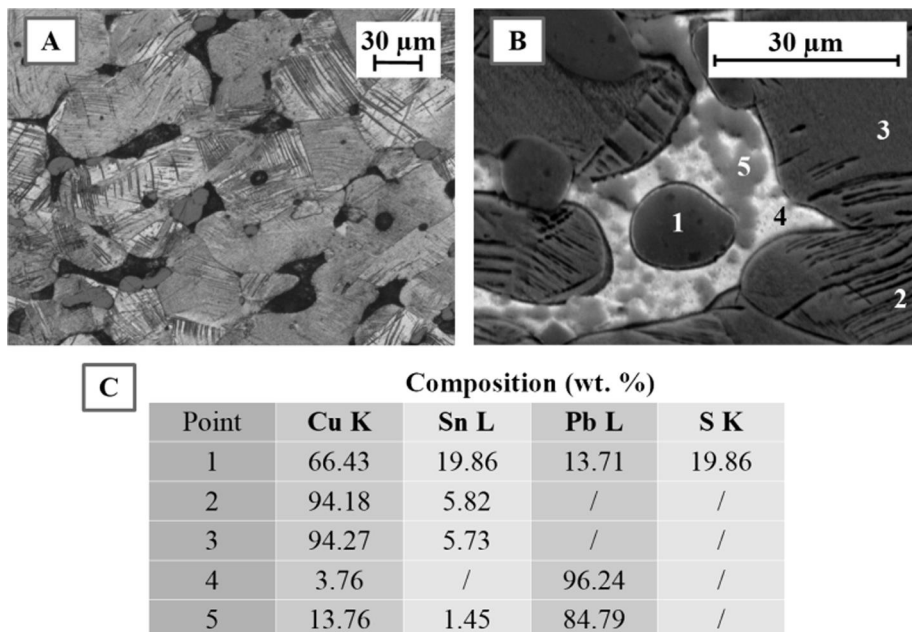
Fig. 3. Coin 1: microstructure of coin's bulk after etching in aqueous FeCl 3 solution. OM-Leica image (A); SEM-FEI backscattered electron image (B); indication of the EDS punctual analyses with corresponding EDS composition (C).
