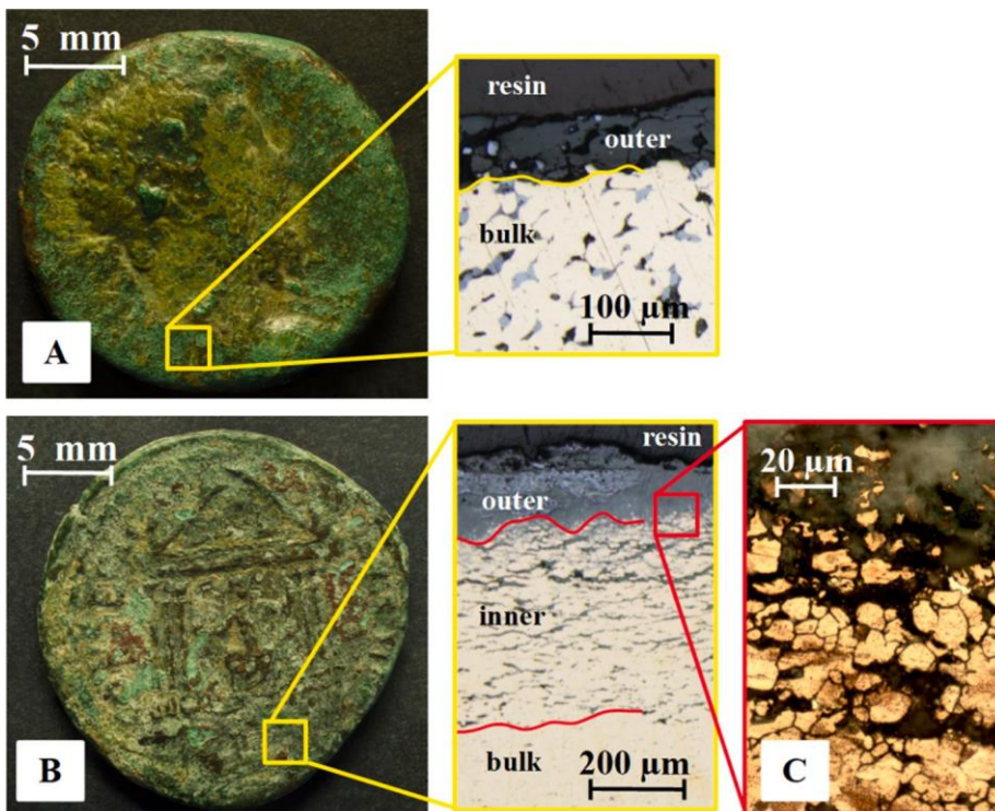
Fig. 5. High-resolution coin photographs and OM cross-section images of the corrosion product structures: (A) Coin 1 and related bright-field OM-Olympus
