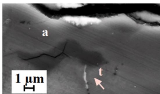
Fig. 13. Particulars (from Fig. 11) of the outer corrosion products layer of Coin 2, non-cleaned and laser-cleaned Test 2 cross-sections: FESEM-Supra-secondary electron images and respective punctual EDS analyses (pink arrows and letters highlight specific particulars points of analysis; amounts expressed in wt.%).
