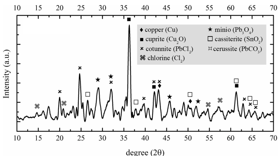
Fig. 10. XRD patterns collected on non-treated surfaces of Coin 2.
