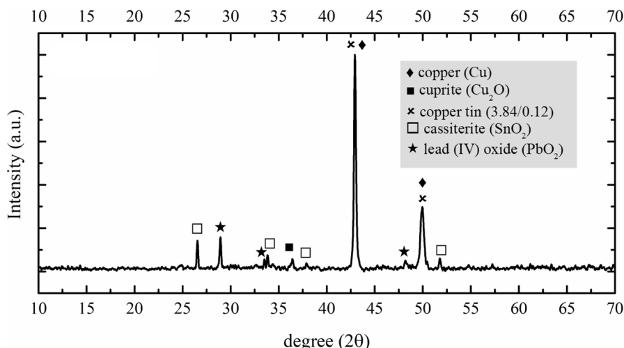
Fig. 7. XRD patterns collected on non-treated surfaces of Coin 1.
