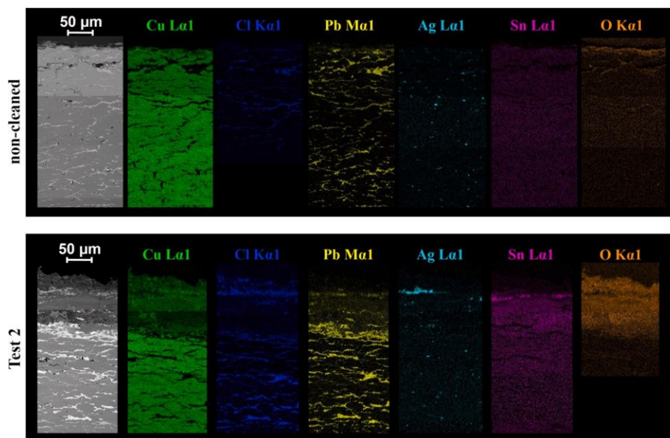
Fig. 12. FESEM-Merlin-EDS maps of non-cleaned and laser-cleaned Test 2 cross-sections of Coin 2.
