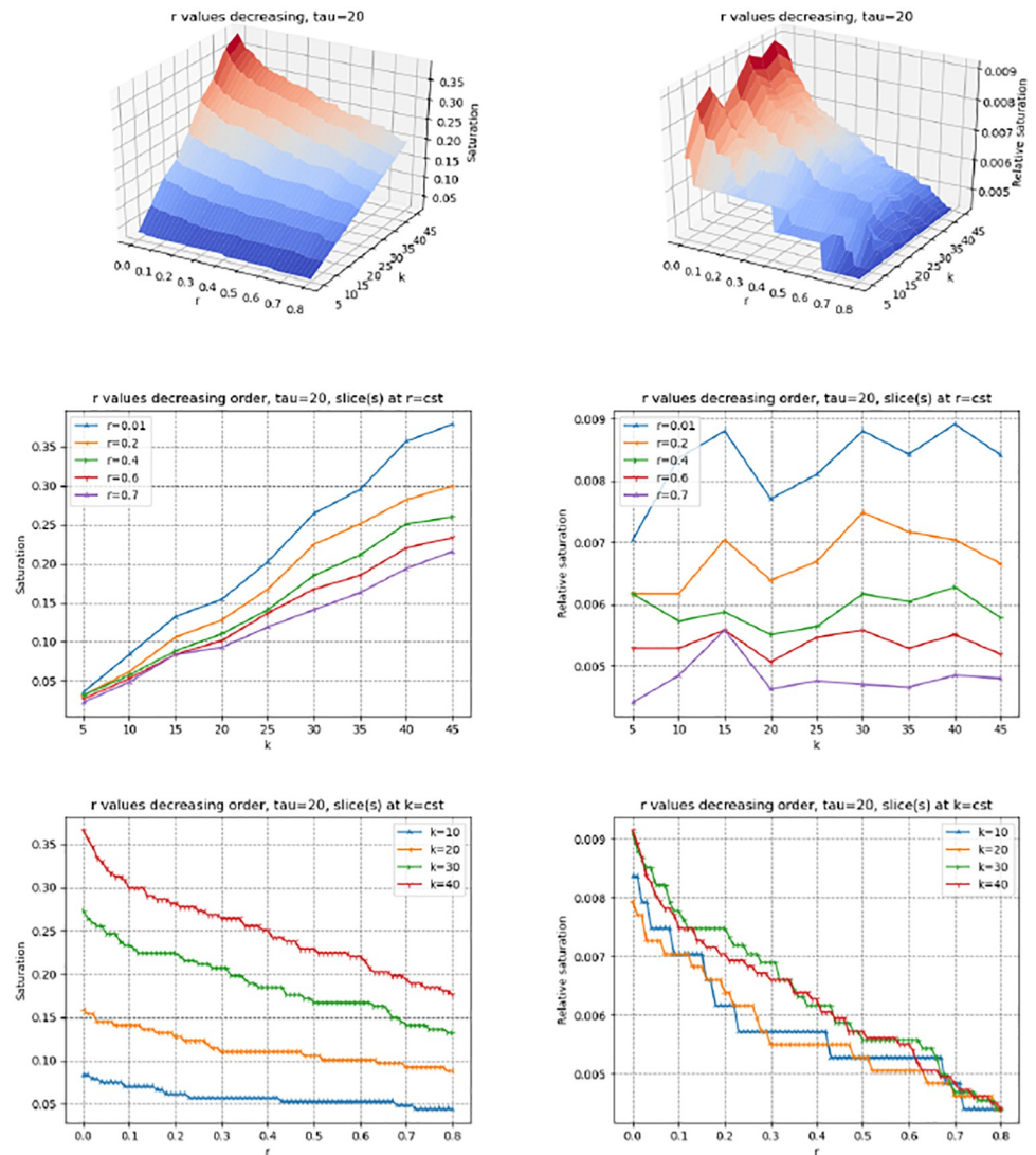
Fig 3. (Genetrack) saturation plots (Def. 5) for \tau = 20 . Values of r processed in decreasing order. (Left column) Saturation index and slices at r = cst and k = cst (See Eq 9) (Right column) Relative saturation index and slices at r = cst and k = cst (See Eq 10).
