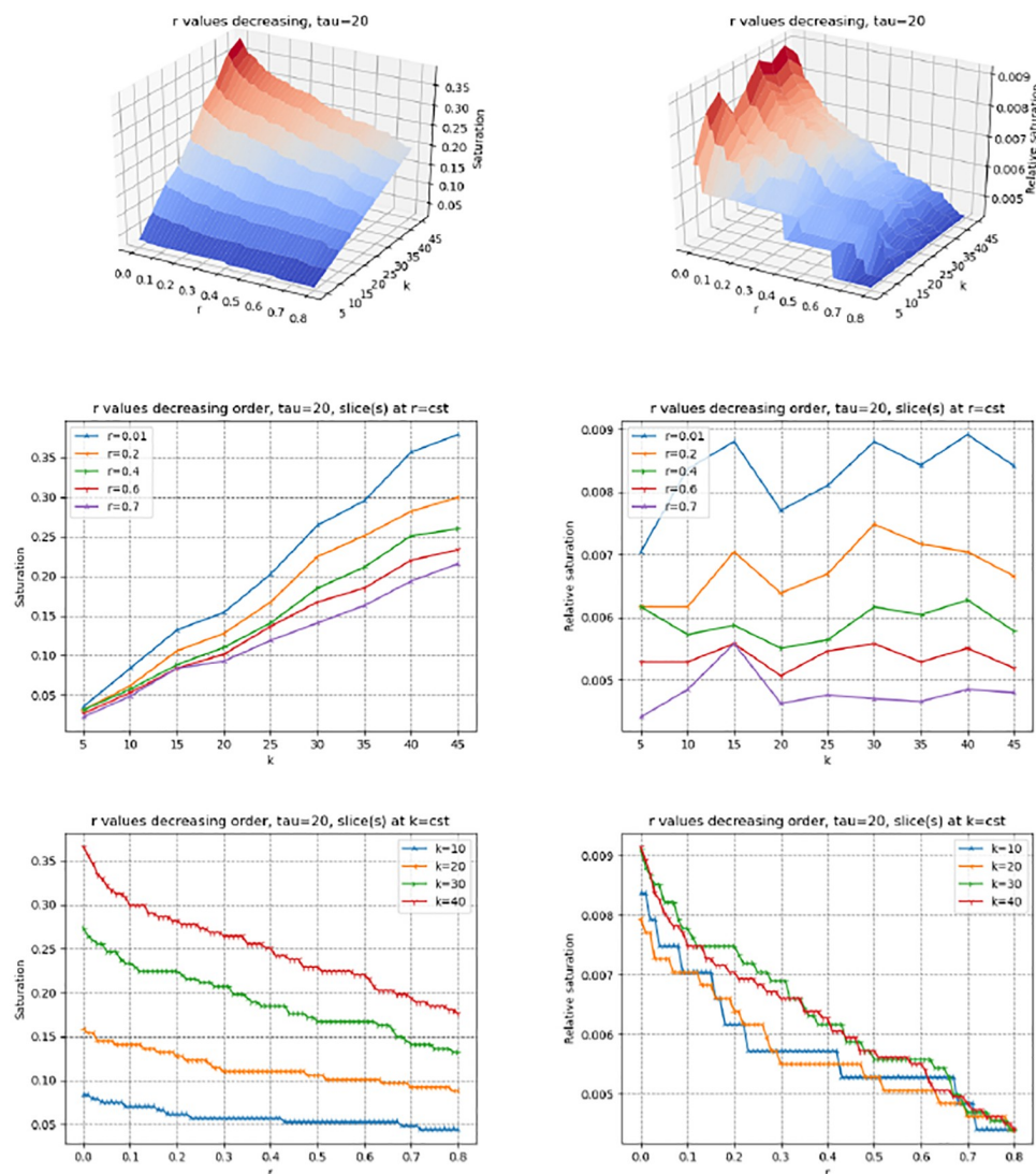
Fig 3. (Genetrack) saturation plots (Def. 5) for \tau = 20 . Values of r processed in decreasing order. ( Left column ) Saturation index and slices at r = cst and k = cst (See Eq 9) ( Right column ) Relative saturation index and slices at r = cst and k = cst (See Eq 10).
