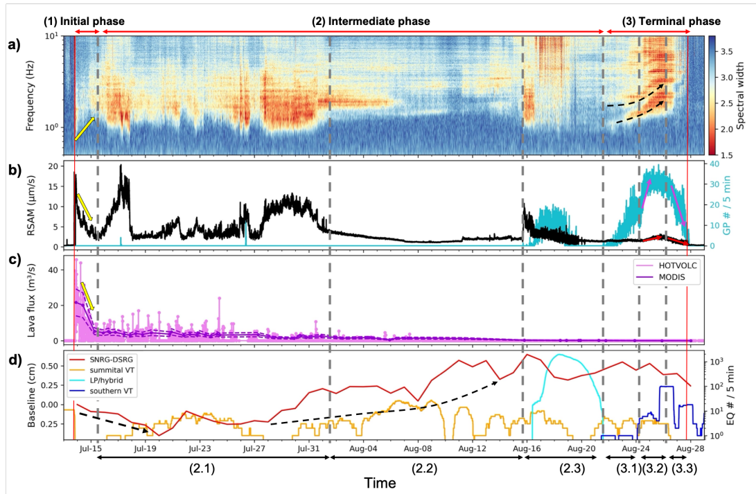
Figure 6: Co-eruptive tremor fluctuations during the long-lived July-August 2017 eruption. a) Covariance matrix spectral width as a
