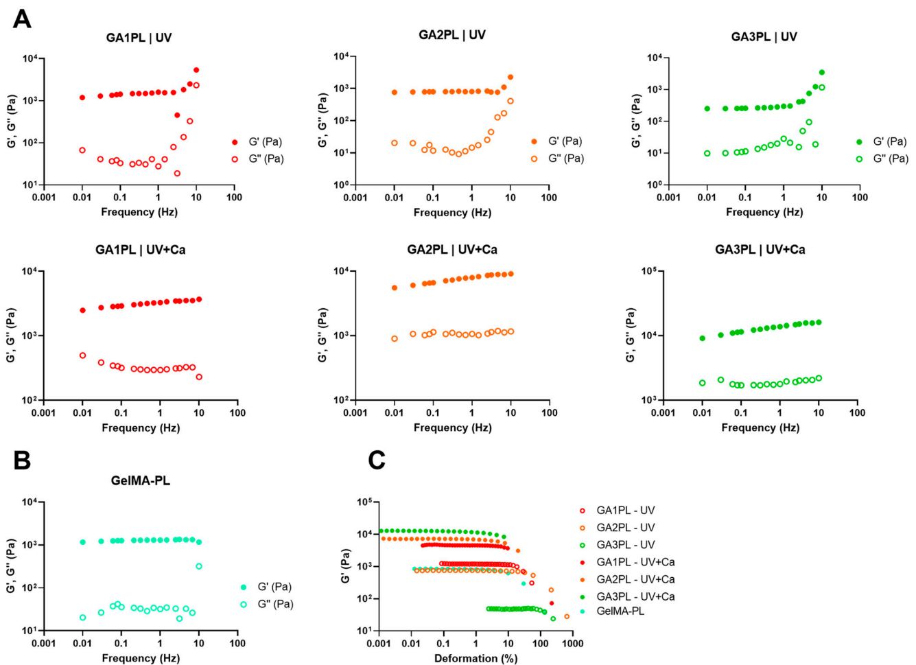
Figure 2. Rheological analysis of G x PL/GelMA-PL gels at different alginate concentrations (0–3% w/v ). (A,B) Mechanical spectra obtained from frequency sweep analyses of gels represented as the elastic ( G' ) and viscous ( G'' ) moduli over frequency (Hz) (colored full dots: G' ; colored empty dots: G'' ). (C) Elastic modulus ( G' ) over deformation of gels before (UV-only) and after calcium crosslink (UV + Ca) (colored empty dots: UV-only gels; colored full dots: UV + Ca gels). Experimental conditions: GelMA, 5.5% w/v ; alginate, 1–3% w/v ; LAP, 0.1% w/v ; human platelet lysate, 50% v/v . Frequency and stress sweep experiments were performed at T = 37 °C.
