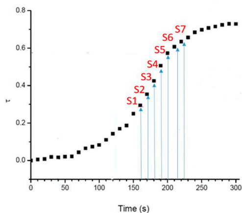
Figure 7. Sampling window from graph plotting the alkene conversion versus time.
