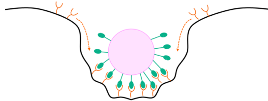
Figure 4 Displacement of the receptors to the contact region during the wrapping of the NP.
