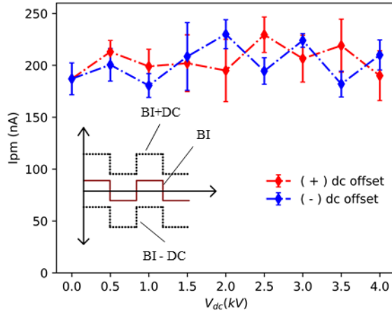
Fig.7. I_{pm} ( \tau = 0.2 s) measured with dc prestress V_{dc} superposed to 6kV pp bipolar impulses ( t_r = 0.28 \mu s, F = 50 Hz).
