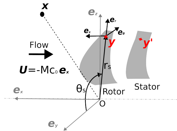
Figure 2. Main coordinate system
