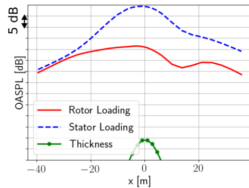
Figure 6. OASPL directivities
