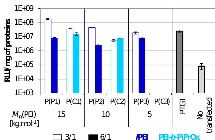
Figure 8. Transfection efficiency of polyplexes. HepG2 cells were transfected for 4 h with polyplexes of lPEI (P(Px)) and PEI-b-PiPrOx (P(Cx)) containing 2.5 \mu\text{g} of pTG11033 with WR_{\text{PEI}} 3/1 and 6/1. The luciferase activity was expressed as relative light unit (RLU) per mg protein after 48 h. The values showed average of three independent experiments. (PTG1: commercial reference from Polytheragene®).
