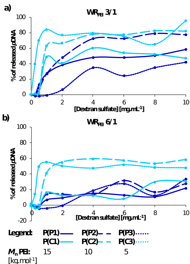
Figure 6. Percentage of released pDNA in function of the dextran sulfate concentration for homopolymers l PEI (P x ) and copolymers PEI- b -PiPrO x (C x ) with WR PEI (a) 3/1 and (b) 6/1.
