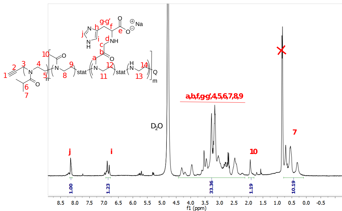
Figure S2: ^1\text{H} NMR spectrum of C1-his in \text{D}_2\text{O}
