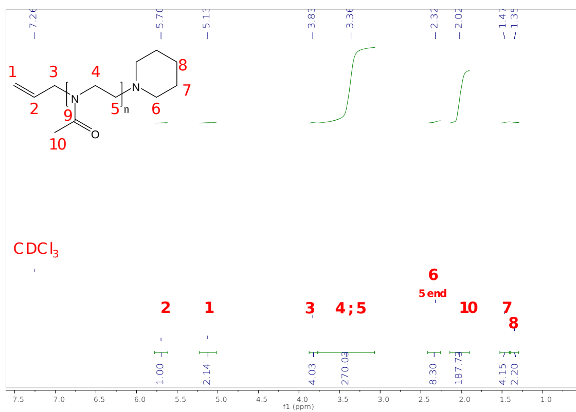
Figure S1: ^1\text{H} NMR spectrum of PMeOx in \text{CDCl}_3
