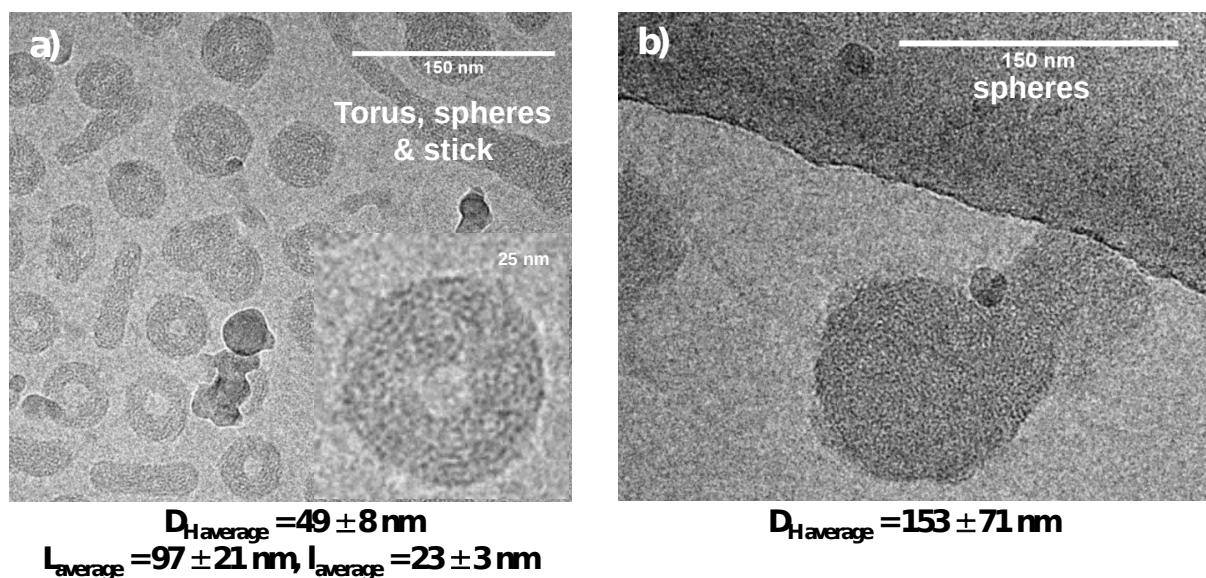
Figure 5. Cryo-TEM pictures of polyplexes obtained with (a) P1 and (b) C2.
