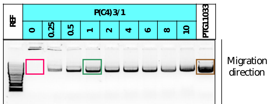
Figure S4: Quantification of the pDNA release with ImageJ
