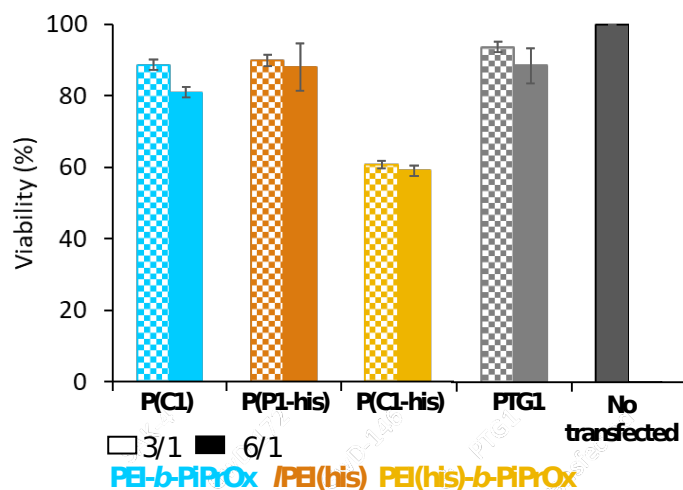
Figure 10. HepG2 cell viability with polyplexes obtained with copolymers without or with histidinylation (C1 and C1-his respectively) and histidinylated homopolymers PEI (P1-his) with PEI block of 15 \text{ kg}\cdot\text{mol}^{-1} at WR_{PEI} 3/1 and 6/1. (PTG1: commercial reference from Polytheragene®)
