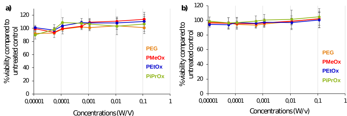
Figure 1. Viability of (a) HeLa and (b) A549 cells. Cells were exposed to PEG and POx at different concentrations from 1.1 \times 10^{-5} to 0.11 W/V. The cell viability was evaluated by MTT assay 24h after exposition and expressed as percentage relative of untreated cells.
