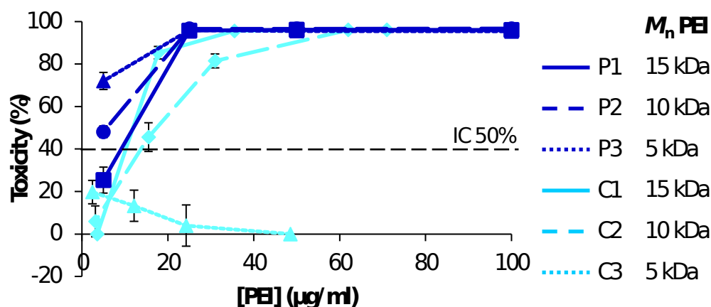
Figure 7. Cytotoxicity of homopolymers PEI (Px) and copolymers PEI- b -PiPrOx (Cx) on HepG2 cells as function of the PEI concentration.
