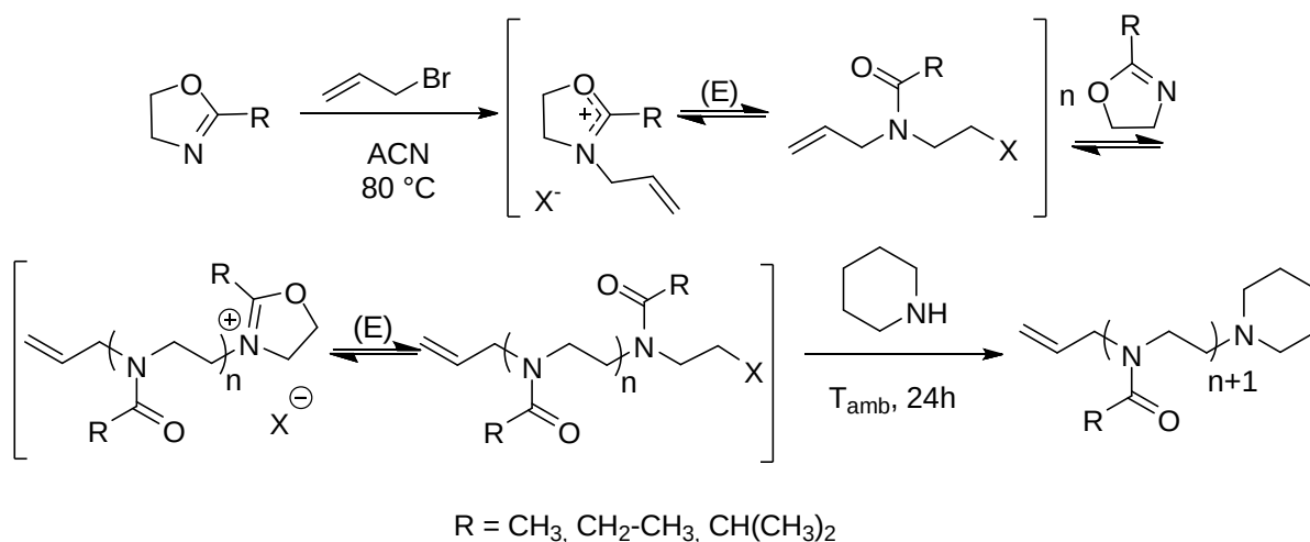
Scheme 1. Synthesis of homopolymers of 2-alkyl-2-oxazoline
