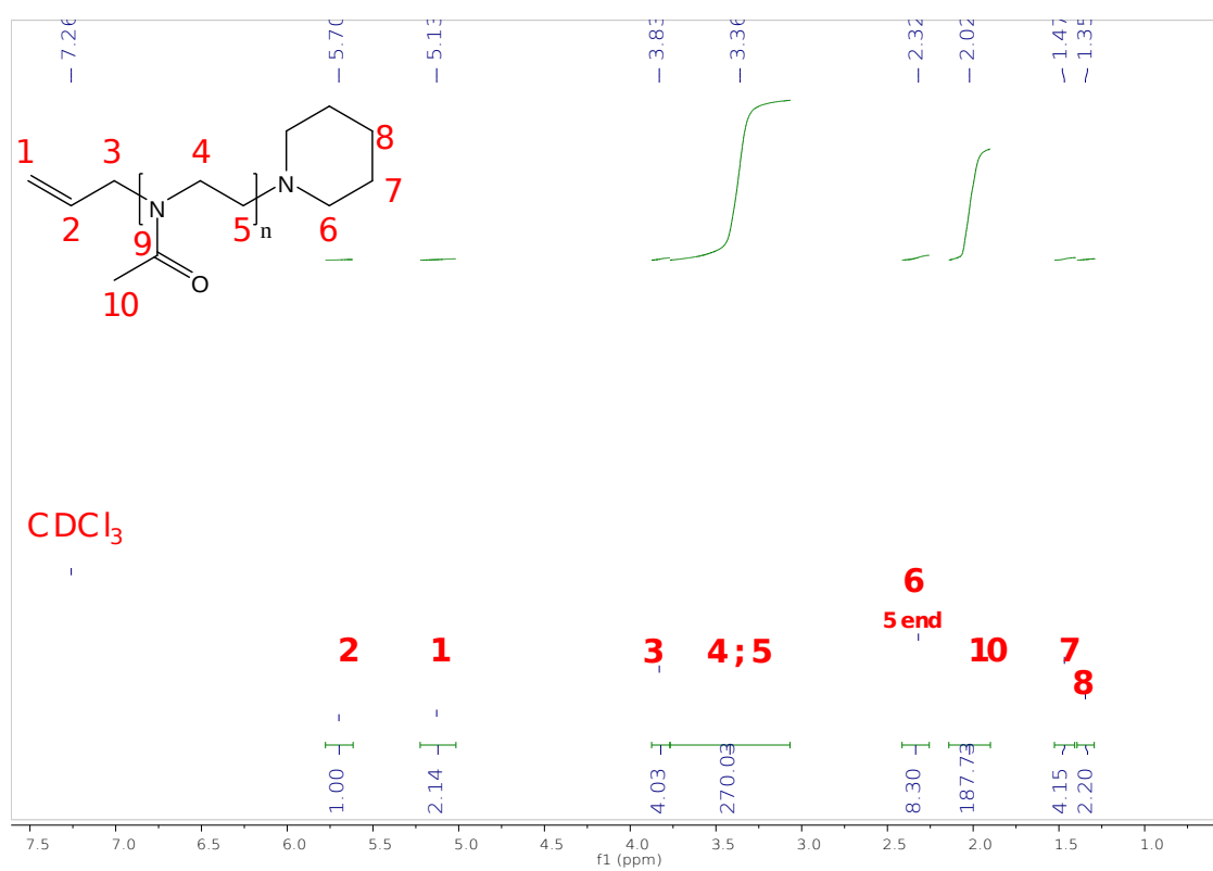
Figure S1: 1 H NMR spectrum of PMeOx in CDCl 3
