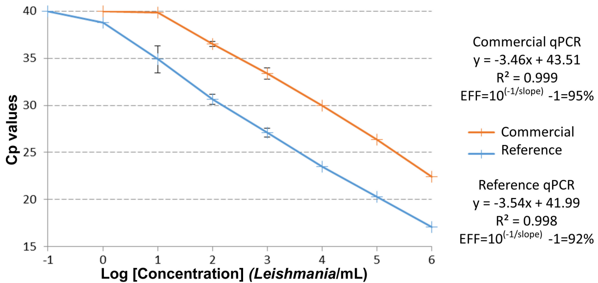
FIG 2 Linearity zone and PCR efficiency (EFF) estimated from the standard curves obtained in the one-tenth serial dilution assays.
