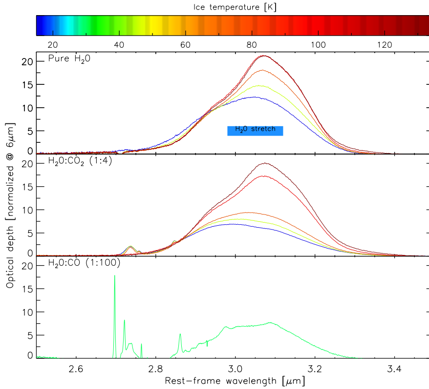
Fig. C.2. Same as Fig. C.1, but showing the stretch mode ( \sim 3 \mu\text{m} ) of the water ice band.
