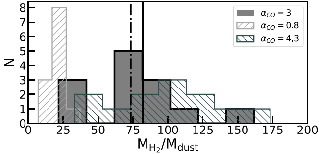
Figure 6. Histogram of the gas-to dust ratio ( M_{\text{gas}}/M_{\text{dust}} ) of our sample, for an \alpha_{\text{CO}} = 3 M_{\odot} (\text{K km s}^{-1} \text{pc}^2)^{-1} , is plotted in solid. We also plot the histograms that result from assumptions of \alpha_{\text{CO}} = 0.8 and 4.3 M_{\odot} (\text{K km s}^{-1} \text{pc}^2)^{-1} for comparison.
