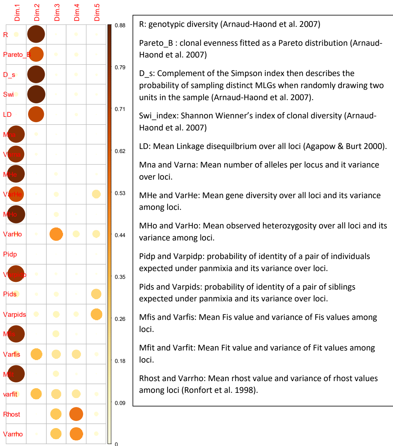
Figure S4: Contributions of population genetic indices to the total variance of genetic diversity in simulated datasets. Contributions of indices to dimensions are reported following the color scale on the right of the matrix.
