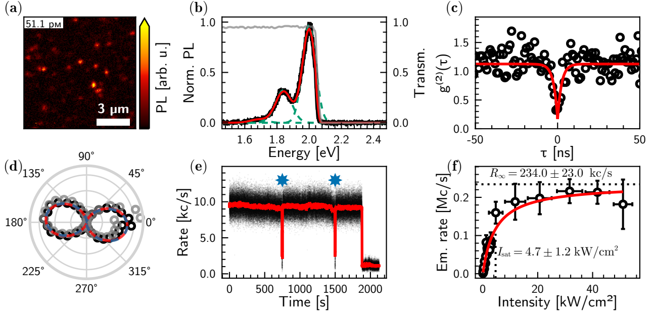
Figure 2: (a) Confocal raster scans of sample with \text{C}_{96}\text{tBu}_8 in PS matrix displaying diffraction-limited emission spots. Concentration in the solution was 54.6 \mu\text{M} . (b) Typical PL spectrum of a single \text{C}_{96}\text{tBu}_8 (solid black), with the corresponding fitted model (solid red). The model includes setup transmission (solid light gray) and three Lorentzian peaks (dashed green). (c) Second-order correlation measurement, excited at 0.15 \text{kW}/\text{cm}^2 . The histogram (black circles) is fitted using a single exponential with a constant added to account for bunching (solid red line). g^{(2)}(\tau) at origin is fitted at 0.17, and the characteristic time of the exponential is 2.43 ns. (d) Emission polarization diagram (black circles) fitted with Malus's law (solid red line) and excitation polarization scan (grey circles) fitted with Malus's law (dashed blue line). The two fit superimpose nearly perfectly. (e) Time trace of the measured emission of a single emitter at excited at 0.15 \text{kW}/\text{cm}^2 . Binning rate is 100 Hz. The moving average over 2 s is plotted in solid red. Manual adjustments of the setup are marked with a blue star. Other variations are attributed to experimental instabilities. (f) Saturation curve of a single \text{C}_{96}\text{tBu}_8 (black circles). The curve is fitted to the model in equation 1, yielding a saturation intensity of 4.7 \pm 1.2 \text{ kW}/\text{cm}^2 and an asymptotic rate of 234 \pm 23 \text{ kc/s} . Signals for Figures (c), (d), (e) and (f) are collected over the whole spectrum in Figure (b)
