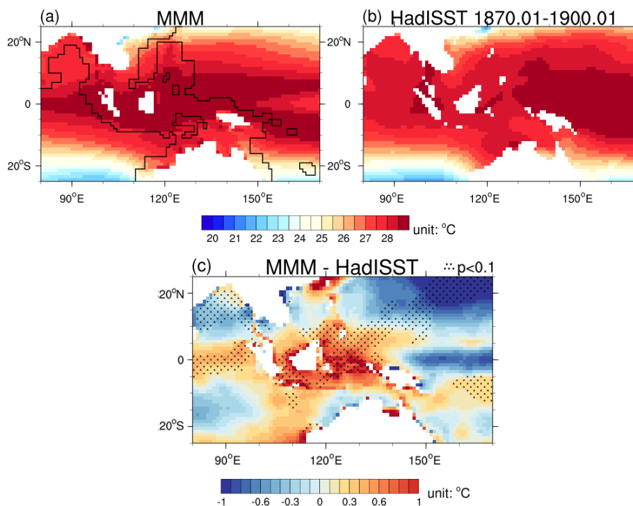
Figure 2. The annual mean sea surface temperature (SST) over the MC from the (a) PlioMIP2 multi-model ensemble mean (MMM) for the preindustrial ( E^{280} ), (b) HadISST1 reanalysed SSTs between January 1870 to January 1900 and (c) their difference. White shading indicates the grid boxes that are land for all the models. In panel (a), grid boxes outside the black lines are ocean grid boxes for all the models. Stippled areas show significant differences, according to a one-sample t test, at the 90 % confidence level.
