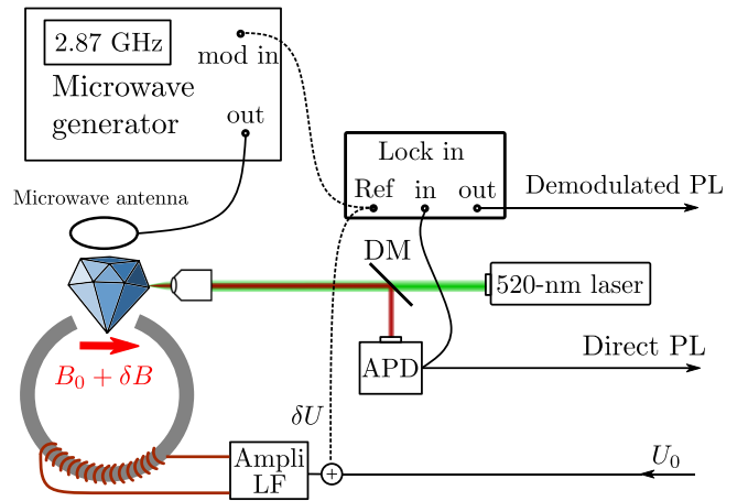
FIG. 2. Experimental setup. Diamonds are subjected to a green laser and a magnetic field in the hundreds of gauss range. PL in the \mu\text{W} range passes through a dichroic mirror (DM) and is detected on an avalanche photodiode (APD).
