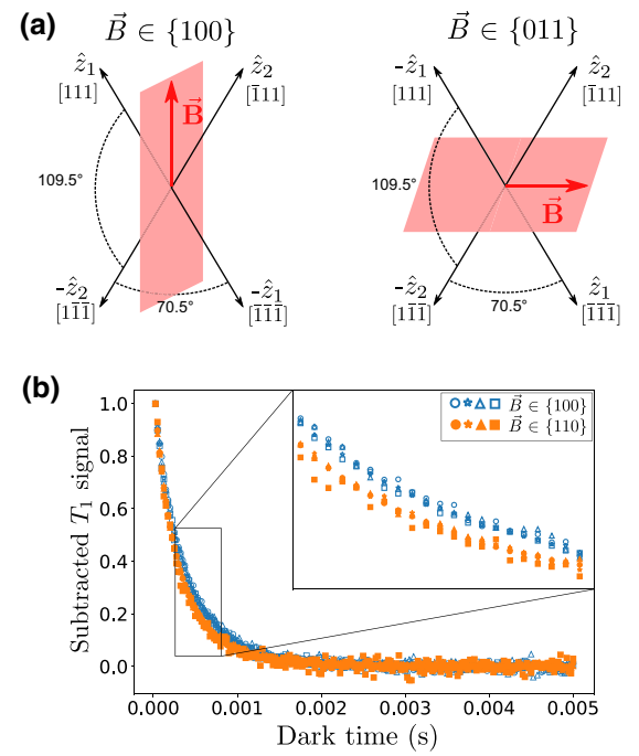
FIG. 11. (a) Geometrical representation of two N- V classes, and the two possible planes where the magnetic field has the same projection on both classes. Positive \hat{z}_i direction is chosen so that \mathbf{B} \cdot \hat{z}_i > 0 . (b) T_1 measurement on a two-class resonance. Eight different magnetic field angles were employed on the same sample: 4 times in the \{100\} plane (blue unfilled symbols) and 4 times in the \{110\} plane (orange filled symbols). Inset, magnification of the 0.3–0.8-ms region. Sample HPHT-150-2.
