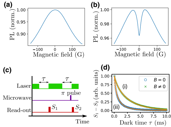
FIG. 7. (a),(b) Photoluminescence from N- V -center ensembles as a function of a magnetic field applied in an arbitrary direction for sample CVD-1 with [N-V] \approx 50 ppb and for sample HPHT-150-1 with [N-V] \approx 3 ppm, respectively. (c) Sequence used to measure the spin lifetime. (d) Traces (ii) and (i) are the spin-relaxation signals, S_1 - S_2 , measured for sample HPHT-150-1 at zero and nonzero magnetic fields, respectively. Fitting procedure (orange plain line) is described in the text.
