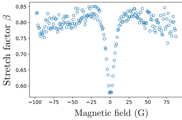
FIG. 9. Best stretch factor, \beta , for a T_1 fit of the form f(\tau) = A \exp\left(-\left(\frac{\tau}{T_1}\right)^\beta\right) as a function of an arbitrarily oriented magnetic field amplitude. Sample HPHT-150-1.
