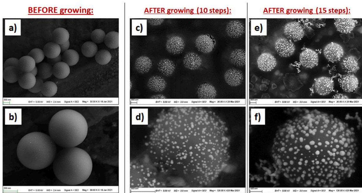
Fig. 4. Silica-gold nanoparticles achieved from the gold-seeded silica particles (a–b) with 10 (c–d) or 15 (e–f) successive additions of trisodium citrate and \text{HAuCl}_4 at 90°C (no centrifugation).
