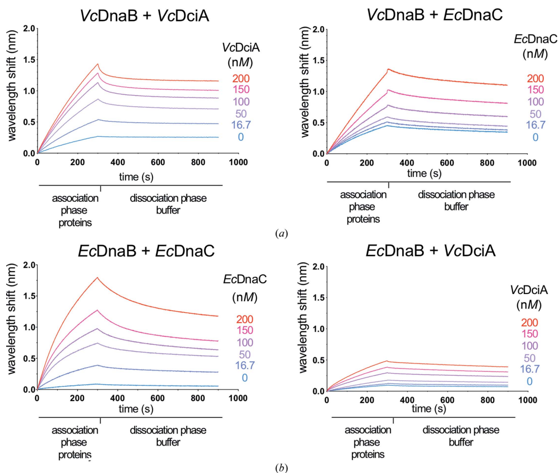
Figure 3 VcDciA and EcDnaC loaders are functionally interchangeable in vitro . Biolayer interferometry (BLI) analysis using a biotinylated oligonucleotide (50 nucleotides) immobilized onto the surface of an SA-coated probe by its 3' extremity (see Section 2). Association was performed with the indicated helicase at a concentration of 100 nM during 300 s in a buffer solution containing ATP and MgCl 2 . Dissociation was assessed in the same buffer for 600 s. Increasing loader concentrations (from 0 to 200 nM in subunits; blue to red) were analyzed. The experiments were carried out in duplicate; only one is presented. (a) VcDnaB binding on ssDNA in the presence of VcDciA (left) or EcDnaC (right). (b) EcDnaB binding on ssDNA in the presence of EcDnaC (left) or VcDciA (right).
