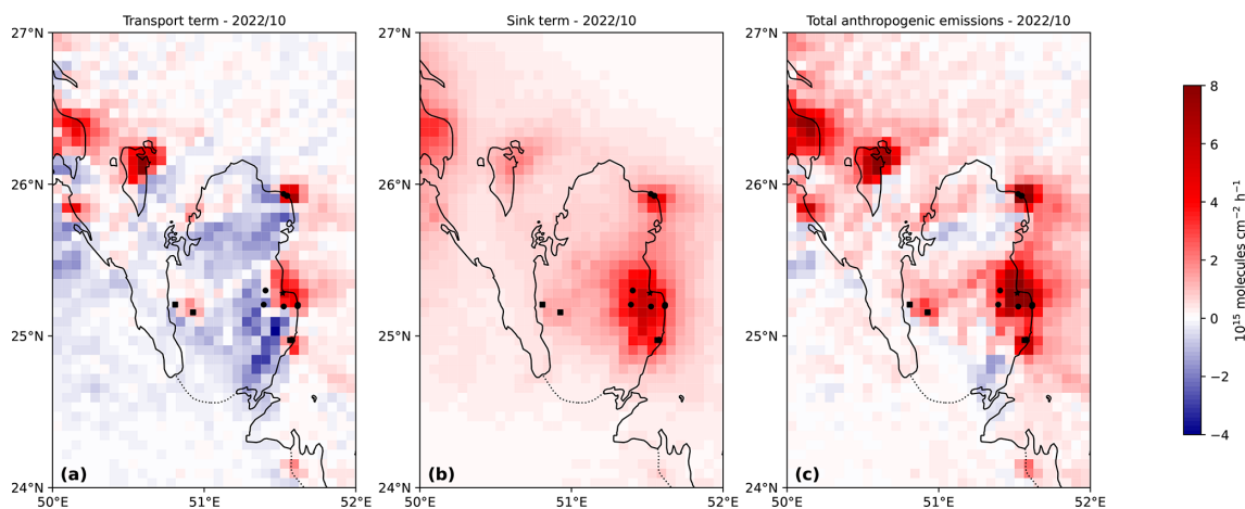
Figure 5. Mean NO x emissions above Qatar (13:30): transport term (a), sink term (b) and resulting emissions (c) for October 2022. Power plants are denoted with dots, cement plants are denoted with squares, and Doha's city centre is denoted with a star.
