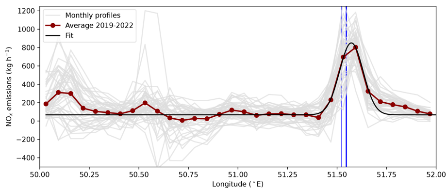
Figure 13. Zonal cross-sections of 13:30 NO x emissions at the latitude of Ras Laffan power plants. The average profile for 2019–2022 is displayed in red, and the corresponding Gaussian fit is displayed in black. Individual monthly profiles are displayed in light grey. The positions of the three power plants are marked with vertical blue lines.
