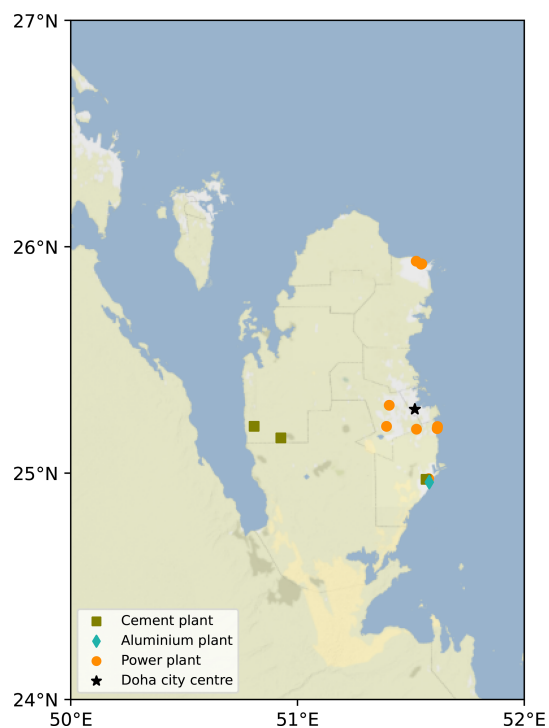
Figure 1. Location of the main industrial facilities (cement kilns, power plants and aluminium smelters) in Qatar. Urban areas are displayed in grey, and Doha's city centre is denoted with a star. Industrial facilities and cities in other countries are not displayed. Map tiles by Stamen Design under CC BY 3.0. Data from © OpenStreetMap contributors.
