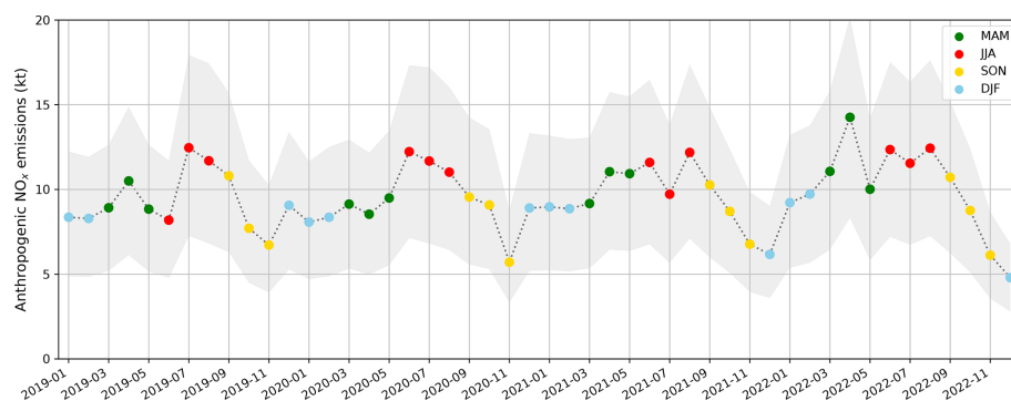
Figure 10. Total TROPOMI-derived anthropogenic NO x emissions in Qatar from 2019 to 2022 using the flux-divergence method. The colours are used to illustrate seasonal variations (green: MAM; red: JJA; yellow: SON; blue: DJF).
