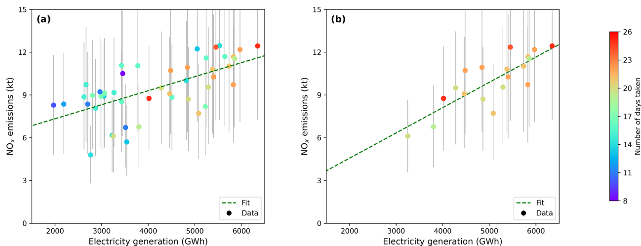
Figure 12. Comparison between monthly TROPOMI-derived NO x emissions for the entire Qatar territory and corresponding electricity generation according to Planning and Statistics Authority reports. A linear regression between the two datasets is displayed with a dashed green line. (a) All months in the period 2019–2022 are included. (b) Months that are included are those for which inferred total emissions have been obtained with an averaging of 18 daily emissions or more. The colour scale represents the number of days involved in the calculation of points.
