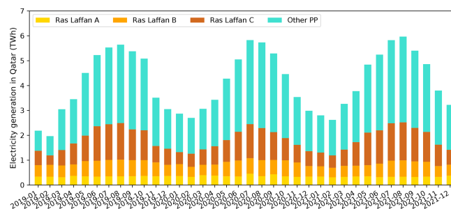
Figure 11. Electricity generation in Qatar from 2019 to 2021 according to the Planning and Statistics Authority reports. Generation from the three Ras Laffan power plants in the northeastern part of the country, is displayed in yellow, orange and brown, while generation from other power plants is displayed in light blue.
