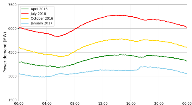
Figure 9. Monthly mean power demand in Qatar for 4 different months in 2016–2017.
