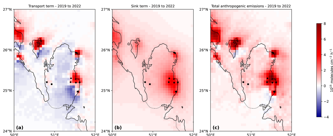
Figure 6. Mean NO x emissions above Qatar (13:30): transport term (a), sink term (b) and resulting emissions (c) for the 2019–2022 period. Power plants are denoted with dots, cement plants are denoted with squares, and Doha's city centre is denoted with a star.
