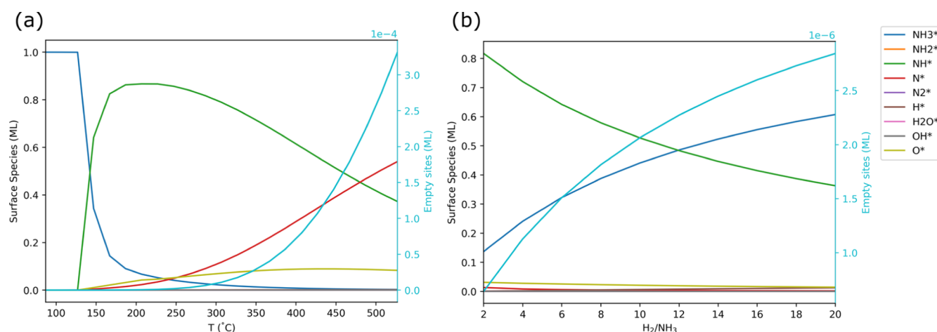
Figure 11. Predicted coverage obtained from microkinetics in combination with the energy barriers computed at the DFT level (Figure S6) as a function of (a) temperature at a \text{H}_2/\text{NH}_3 ratio of 1.0 and (b) \text{H}_2/\text{NH}_3 ratio at a temperature of 200 °C. The adsorbed species \text{OH}^* , \text{H}_2\text{O}^* , \text{NH}_2^* , \text{N}_2^* , and \text{H}^* have negligible coverage at \text{H}_2/\text{NH}_3 = 1.0 with increasing temperature; \text{N}^* and \text{O}^* become negligible with the increasing \text{H}_2/\text{NH}_3 ratio. The evolution of free sites is shown on the twin axis in cyan color.
