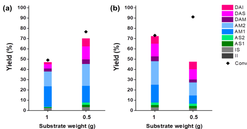
Figure 7. Conversion of isomannide IM and product distribution at 1 and 0.5 g IM under (a) 5 bar and (b) 10 bar H 2 . Other reaction conditions: 15 mL NH 3 ·H 2 O (25 wt %) (pH = 12), 0.2 g Ru/C catalyst, 180 °C, and 18 h.
