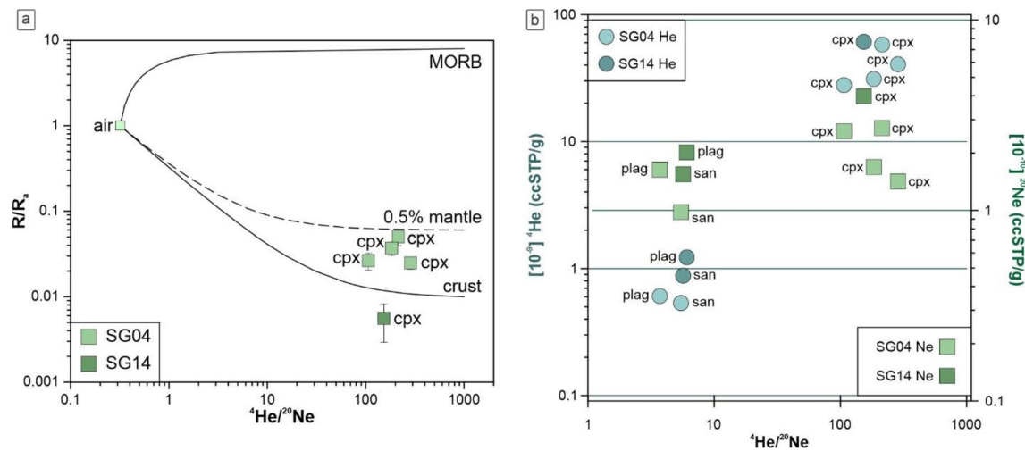
Fig. 7 Noble gas isotopic systematics of the studied mineral phases. A. R/R_a vs. ^4\text{He}/^{20}\text{Ne} plot. B. ^4\text{He} and ^{20}\text{Ne} concentrations vs. the ^4\text{He}/^{20}\text{Ne} ratios with their uncertainties (equivalent with the size of the rectangle/circle unless marked otherwise). The measured separates are clinopyroxene (cpx), sanidine (san) and plagioclase (plag)
