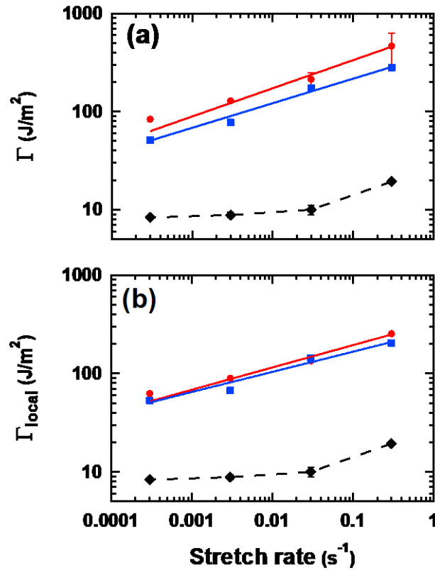
5 Figure 12. Fracture energy \Gamma (a) and effective fracture energy \Gamma_{\text{local}} (b) as a function of stretch rate, 6 for chemical gels and dual crosslink gels. Red circles: P(AAm-co-VIm)-Ni 2+ gel, blue squares: 7 P(AAm-co-VIm)-Zn 2+ gel, black diamonds: chemical gel.
