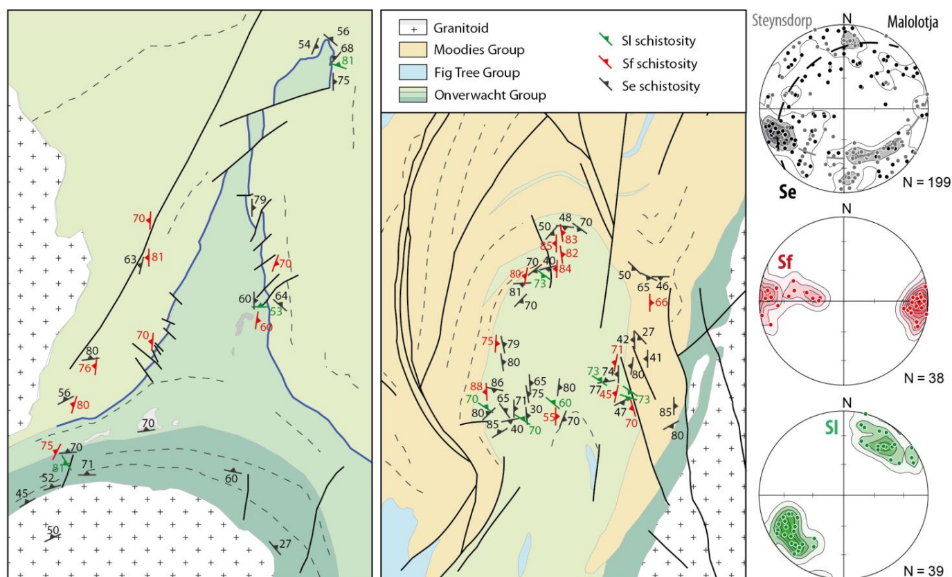
Figure 5. Structural map of the Steynsdorp antiform and the Malolotja synform with Se, Sf, and SI cleavage distribution. Planar structural data are presented as poles to planes on equal-area lower hemisphere projections, with the associated main direction (dashed great circles). The background maps are two inset views of Figure 3 focused on the Steynsdorp (left map) and Malolotja (right map) sectors.
