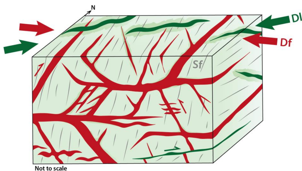
Figure 16. Synthetic sketch illustrating the distribution of the mineralised (red) and barren (green) vein system at the outcrop scale. Note the coexistence between horizontal and steeply dipping westward and eastward veins. Both have N–S and NNW–SSE strikes, although N–S veins dominate. The red and green arrows display, respectively, the Df and D1 deformations, and the grey line is the Sf schistosity.
