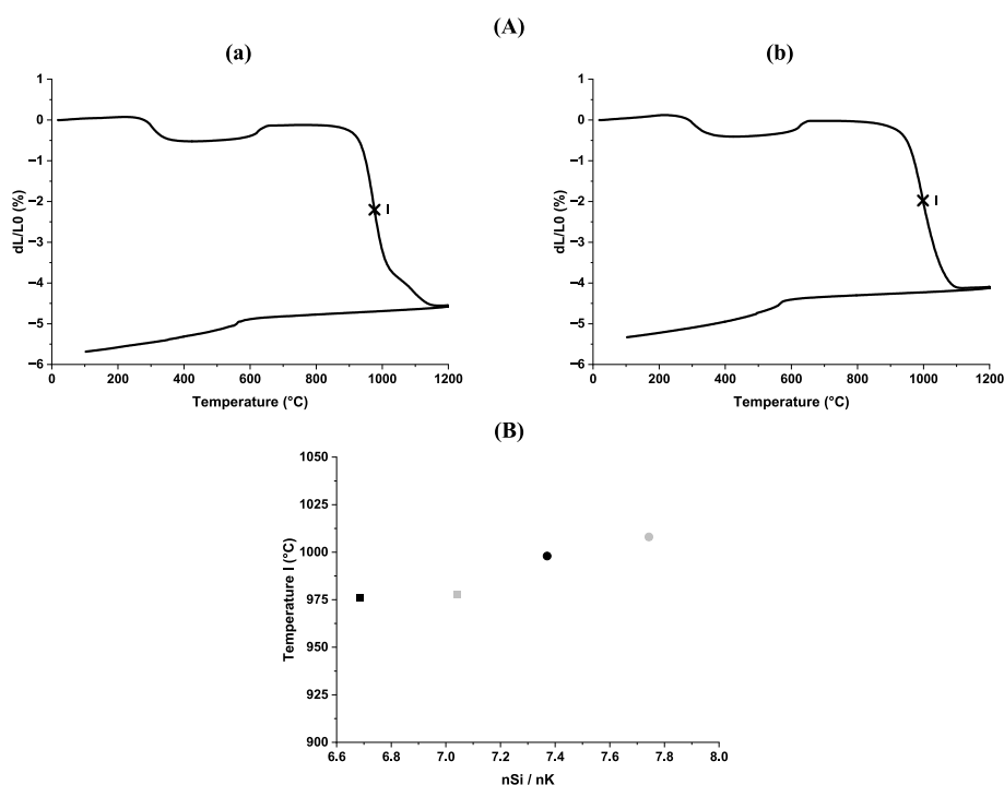
Fig. 6. (A) Dilatometric curves of (a) K 6 MS and (b) K 5 MS samples and (B) evolution of the temperature I according to Si/K molar ratio for (■) K 6 MS, (□) K 6 MSA, (●) K 5 MS, and (○) K 5 MSA samples.
