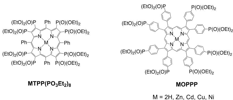
Figure 1. Octa-β-phosphonate-substituted porphyrins investigated in this work.
