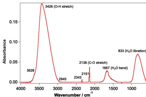
Fig. 1 Infrared spectrum of a mixed CO and water ice dosed on the Au-coated Cu substrate at 18 K. The ice consists of 780 \text{ L}_m of ASW and 13.3% CO.
