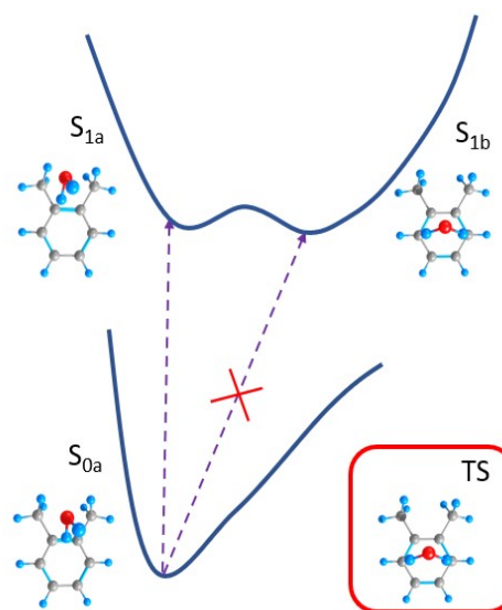
Figure 4 Schematic potential energy diagram for the different o -xylene-H 2 O structures. S_{0a} , S_{1a} and S_{1b} were calculated as minima in the theoretical study, while the transition state was found rather than the expected S_{0b} .
