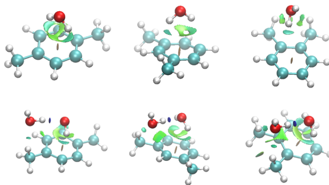
Figure 5 NCI calculated surfaces in the ground state for; top left - p -xylene-H 2 O, top middle - m -xylene-H 2 O, top right - o -xylene-H 2 O, bottom left - p -xylene-(H 2 O) 2 , bottom middle - m -xylene-(H 2 O) 2 , bottom right - o -xylene-(H 2 O) 2 . Repulsive interactions are shown in orange and attractive interactions in blue. Green regions describe both attractive and repulsive interactions.
