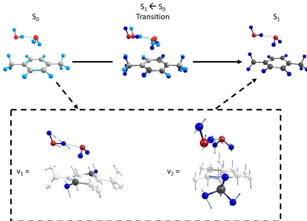
Figure 3 The change in geometry between the p -xylene-(H 2 O) 2 S 0 and S 1 states and the \nu_1 and \nu_2 vibrations that allow the vibronic transition between these states. The structures and vibrations were calculated at the CAM-B3LYP/aug-cc-pVDZ level of theory.
