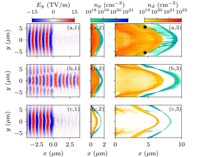
FIG. 4. Laser electric field (*,1), proton ( n_p ) and deuterium ion ( n_d ) number density as the peak intensity reaches the target (*,2) and at the end of the simulation ( \sim 200 fs after the peak intensity) (*,3), obtained by PIC simulations, for three different thickness of the target: 320nm (a,*), 90nm (b,*) and 90nm CD+Au (c,*). Colorbars for proton and deuterium densities are common to (*,2) and (*,3).
