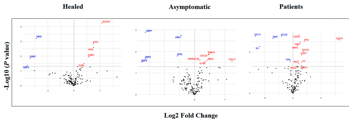
Fig. 2. A Volcano plot depicting Log2 fold changes of the tested genes in the studied groups versus the P values ( -\log_{10} ). Genes with non-significant ( P > 0.05 ) differences are shown as black dots. Using the P -value cutoff, the over- and under expressed DEGs are shown as red and blue dots, respectively.
