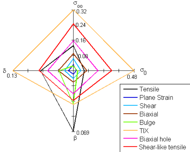
Fig. 17. Sensitivity of S_{obj} to the isotropic work hardening parameters.
