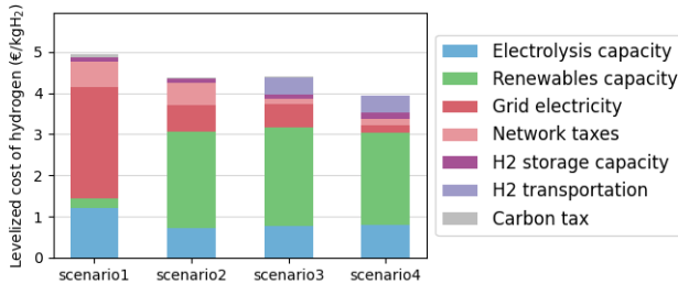
Fig. 3. Comparison of leveled cost of hydrogen breakdown between the different scenarios.
