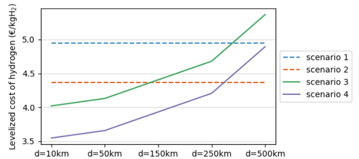
Fig. 4. Sensitivity analysis of the leveled cost of hydrogen to the distance between the industrial zone and the renewable zone
