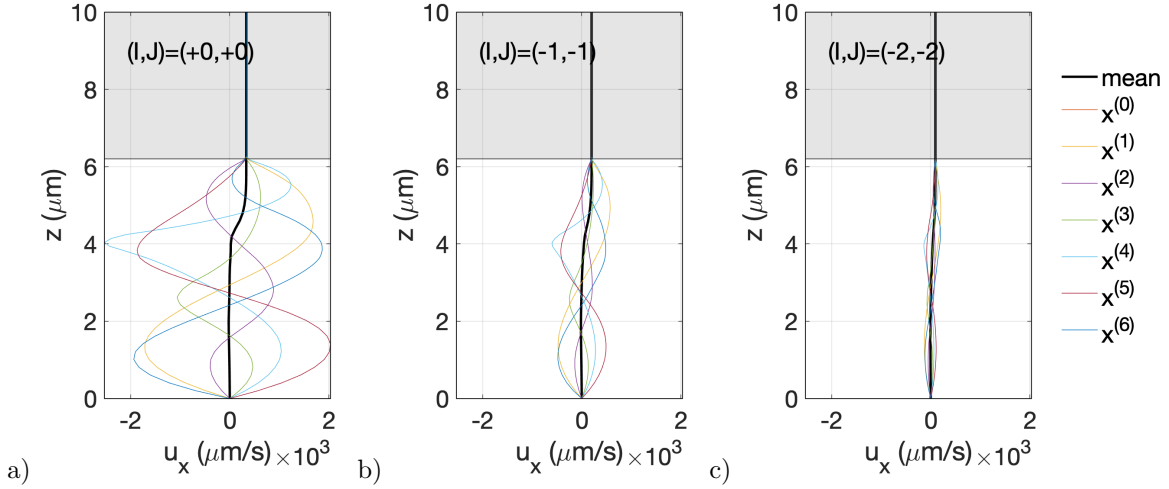
Figure 16: Influence of the density of cilia on the axial velocity, for H = 6.2 \mu\text{m} . All data from Table 2 except for the density of cilia. The axial velocity is averaged in the azimuthal direction y (note that the velocity little varies in this direction) so that we show the following profiles: z \mapsto \overline{u_x^y}(x^{(j)}, z) for different axial positions x = x^{(j)} = j\Delta (with \Delta = 5 \mu\text{m} ). Index (I, J) relates to the following density: d_x = 2^I d_x^0 (axial direction), d_y = 2^J d_y^0 (azimuthal direction), with reference values: d_x^0 = d_y^0 := 3.33 \mu\text{m}^{-1} .
