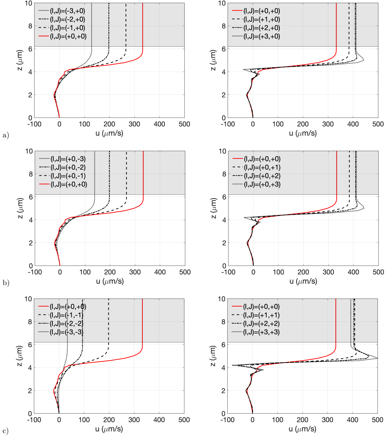
Figure 14: Influence of the density of cilia on the mean axial velocity z \mapsto u(z) := \overline{u}^{x,y}(z) , for H = 6.2 \mu\text{m} . All data from Table 2 except for the density of cilia and the position of the interface. Index (I, J) relates to the following density: d_x = 2^I d_x^0 (axial direction), d_y = 2^J d_y^0 (azimuthal direction), with reference values: d_x^0 = d_y^0 := 3.33 \mu\text{m}^{-1} .
