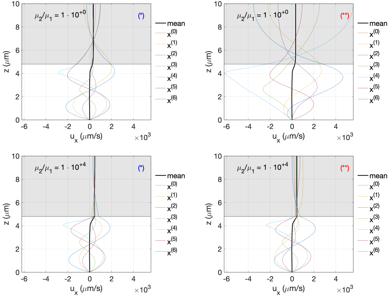
Figure 9: Axial velocity profiles in the radial direction, for different axial positions x = x^{(j)} = j\Delta (with \Delta = 5 \mu\text{m} ). The velocity is averaged in the azimuthal direction y (note that the velocity little varies in this direction) so that we show the following profiles: z \mapsto \overline{u_x^y}(x^{(j)}, z) (*) refers to the standard model with surface tension (hence u_z = 0 is imposed at the PCL-mucus interface) whereas (**) refers to the model in which no surface tension is taken into account (hence u_z is not constrained at the PCL-mucus interface).
