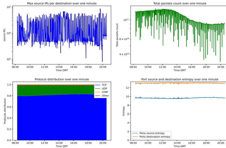
Figure 4: Metrics observed on the captured traffic of a CSP backbone.
