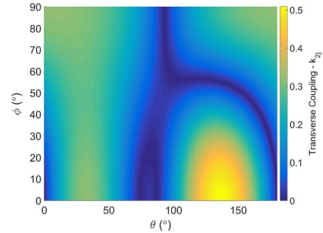
Figure 9. Optimization of effective transverse electromechanical coupling K'_{23} of LiNbO 3 by rotating around axis X by angle \Theta and in the resulting plane XZ' by angle \phi .
