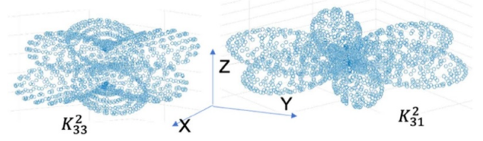
Figure 8. 3D representation of effective K_{33}^2 and K_{31}^2 electromechanical coupling factors of LiNbO 3 . XYZ axes correspond to the standard tensor setting for 3m point group (see table 1).
