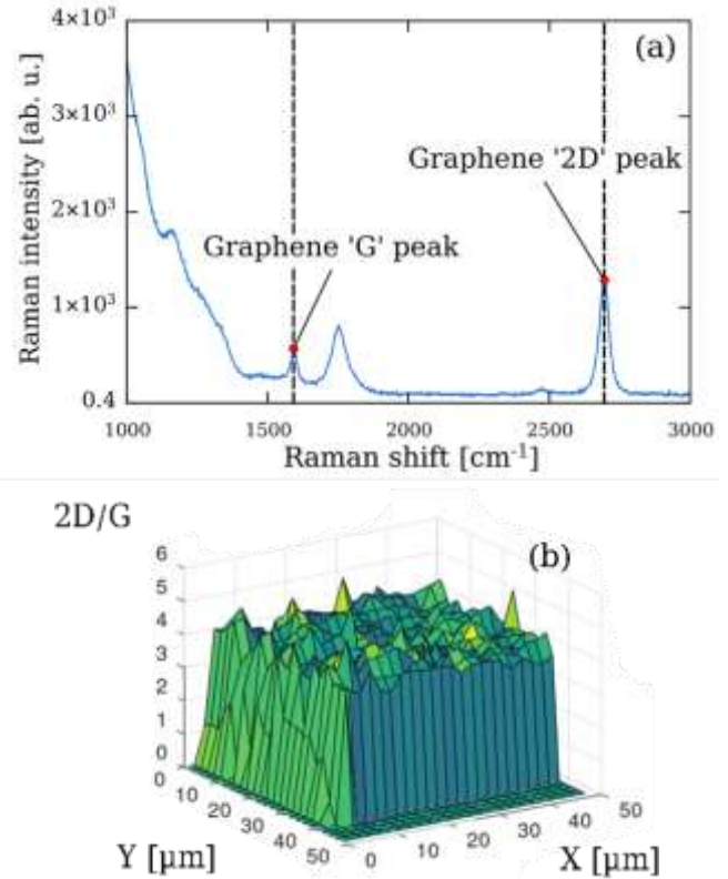
Figure 2: Typical Raman spectrum of graphene transferred to LiNbO 3 (a) and mapping of 2D/G ratio on a 50 \mu\text{m} x 50 \mu\text{m} area (b).
