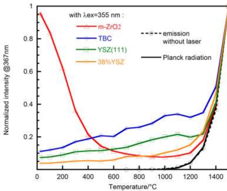
FIGURE 4 Intensity of thermal emission as a function of temperature, measured at 367\text{ nm} with and without laser excitation on m-ZrO 2 , TBC, YSZ(111) and 38%YSZ specimens, in comparison to the calculated Planck's black body radiation at a wavelength of 367\text{ nm} .
