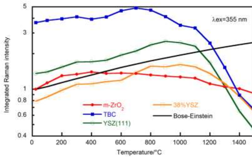
FIGURE 3 Integrated Raman intensity in the spectral range from 150\text{ cm}^{-1} to 850\text{ cm}^{-1} as a function of the temperature for m-ZrO 2 , TBC, YSZ(111) and 38%YSZ, and plot of Bose-Einstein factor.
