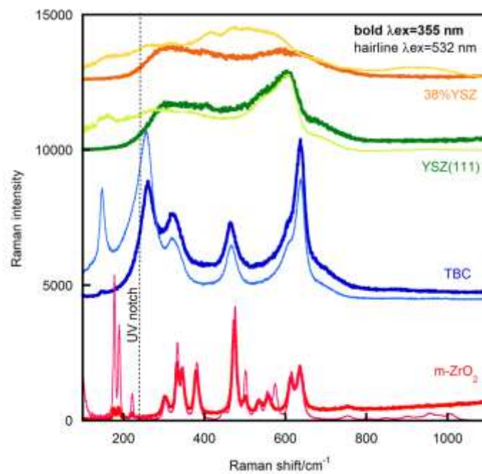
FIGURE 2 Raman spectra at room temperature and measured in the same conditions of m-ZrO 2 , TBC, YSZ(111) and 38%YSZ using 355 nm and 532 nm laser excitation.
