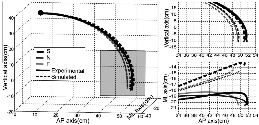
Fig. 6. Simulated finger paths predicted from the best-fitting composite cost (SIComp) and average experimental finger paths for subject S5. Left. 3D finger paths for the three speeds for experimental (plain traces) and simulated (dotted lines) data. Right. The zoomed-in projections of finger paths on the sagittal plane ( top ) and the transverse plane ( bottom ) for the last part of the movement, in order to emphasize differences. In general, fitting errors mainly arose from the discrepancy of trajectories along the ML axis while along the AP axis (main axis of interest here), the simulated trajectories better matched the recorded ones and clearly exhibited a speed dependence.
