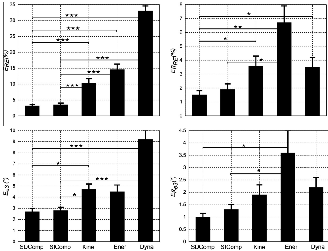
Fig. 7. Reconstruction errors for some relevant movement parameters ( E_{e3} , E_{RE} , E_{KRE} , E_{KRE3} ) for the SDComp, SIComp costs and the three cost elements taken separately. Error values were first averaged across speeds and then across subjects (with standard errors indicated by error bars). Visual inspection reveals that in terms of both E_{RE} and E_{e3} the dynamic cost performs quite poorly compared to the other costs. In terms of E_{KRE} and E_{KRE3} , the energy cost overestimates the speed dependence of RE and e3 parameters. Overall, the kinematic cost performs relatively well but the composite costs perform significantly better than the latter. Importantly, the kinematic cost is also unable to account for any speed-dependence as it predicts constant movement parameters for all speeds. Finally, no significant difference was found between the SDComp and SIComp.
