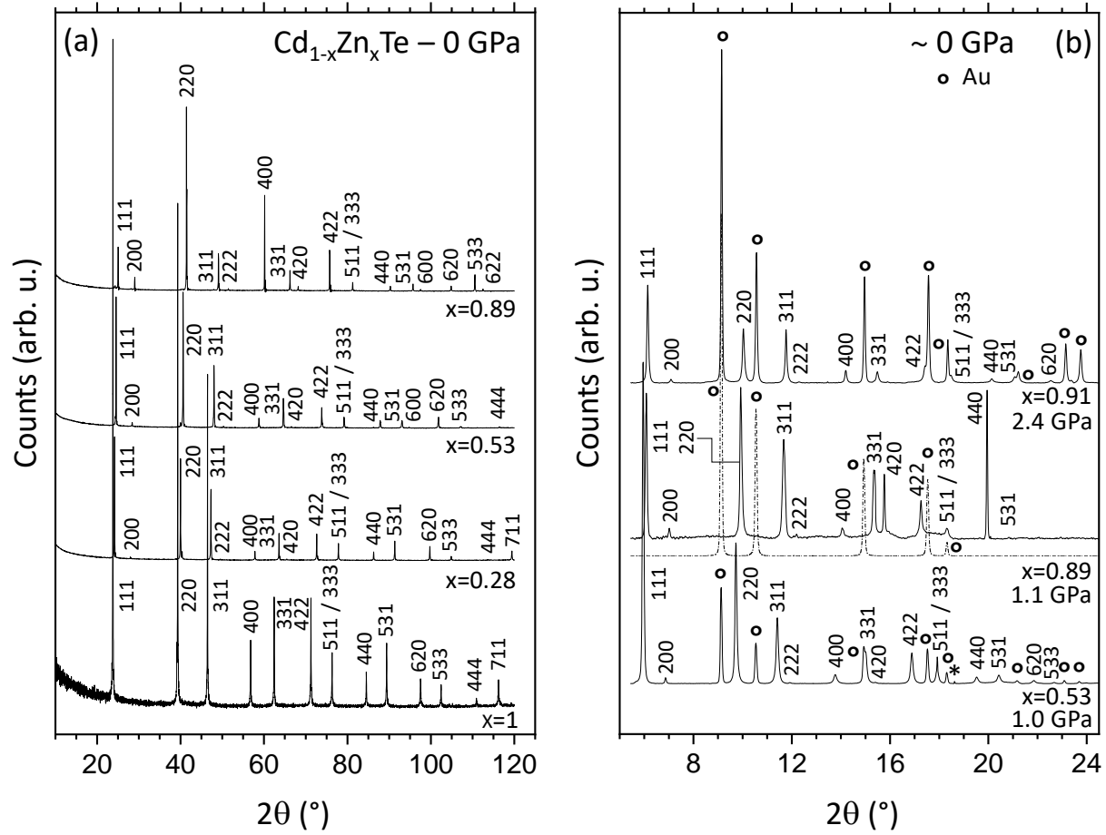
FIG. 2. Cd 1-x Zn x Te X-ray diffractograms. Powder X-ray diffractograms obtained at ambient pressure in laboratory with the Cu K-alpha radiation (a) and at nearly ambient pressure (as specified) on the PSICHÉ beamline of synchrotron SOLEIL with the 0.3738 Å radiation (b). Circles mark diffraction lines due to Au used for pressure calibration. In panel (b) the Cd 1-x Zn 0.53 Te (solid line) and Au (dashed-dotted line) diffractograms were recorded separately. The star refers to a spurious signal.
