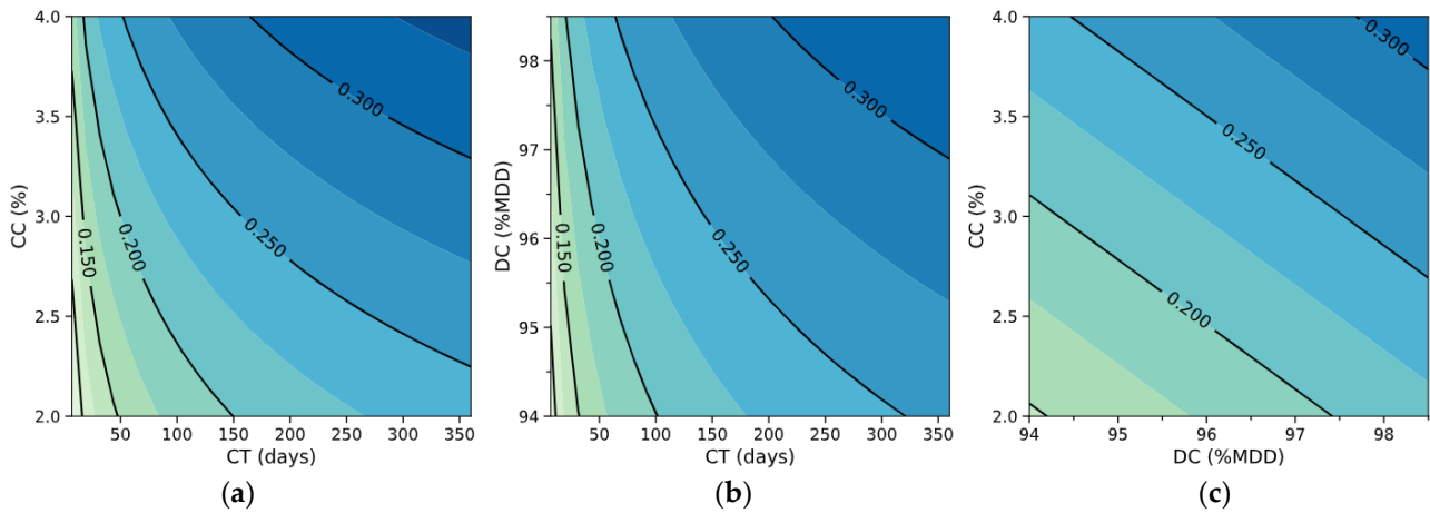
Figure 6. ITS contour plots for mixture B: (a) CT vs. CC (DC = 96% MDD), (b) CT vs. DC (CC = 3%), (c) DC vs. CC (CT = 90 days). Contour lines: ITS, in MPa.
