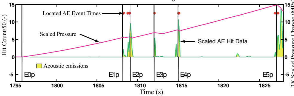
Fig. 26. Evolution of the fluid pressure, electrical potential changes, and acoustic emissions over time. a. The Acoustic Emissions (AEs) and fluid pressure disturbances occur at the same time. b. Self-potential time series recorded at the 32 electrodes of the array. All the signals indicate the existence of 6 hydromechanical disturbances labeled E0 to E5 with the build-up of fluid pressure, the formation of fractures, and the decay of the fluid pressure associated with the flow of the pore water in the cracks. Modified from Haas et al. (2013).
