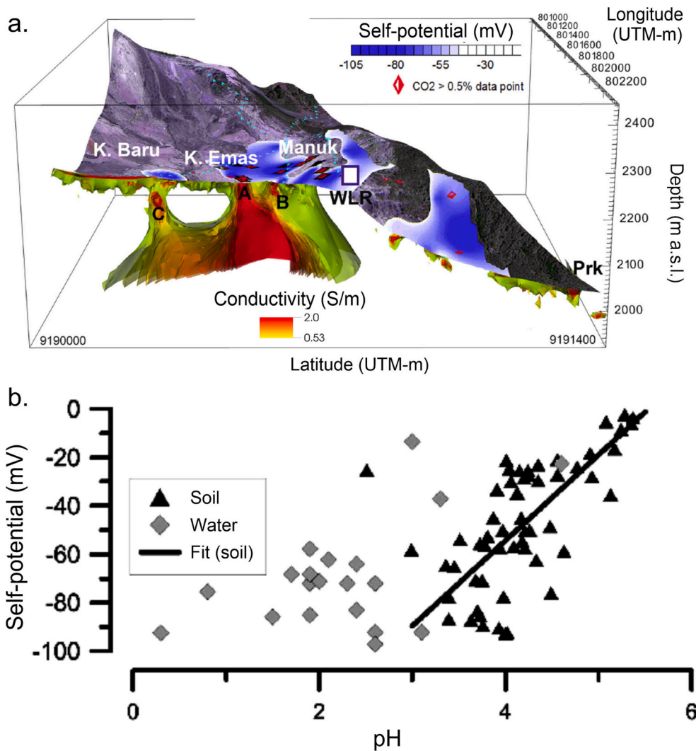
Fig. 24. Papandayan volcano. a. Satellite image superimposed on the digital elevation model of Papandayan volcano with representation of self-potential map below -40 mV and 3D representation of the most conductive areas (above 0.5 S/m) “A”, “B”, “C” associated with the three main fumarole field, K. Emas, Manuk and K. Baru respectively. WLR represents the permanent seismic station and Prk correspond to the parking area. b. Relationship between self-potential and pH measurements performed in soil (black triangles) and pH measurements performed in water (grey diamonds) (Modified from Byrdina et al., 2018).
