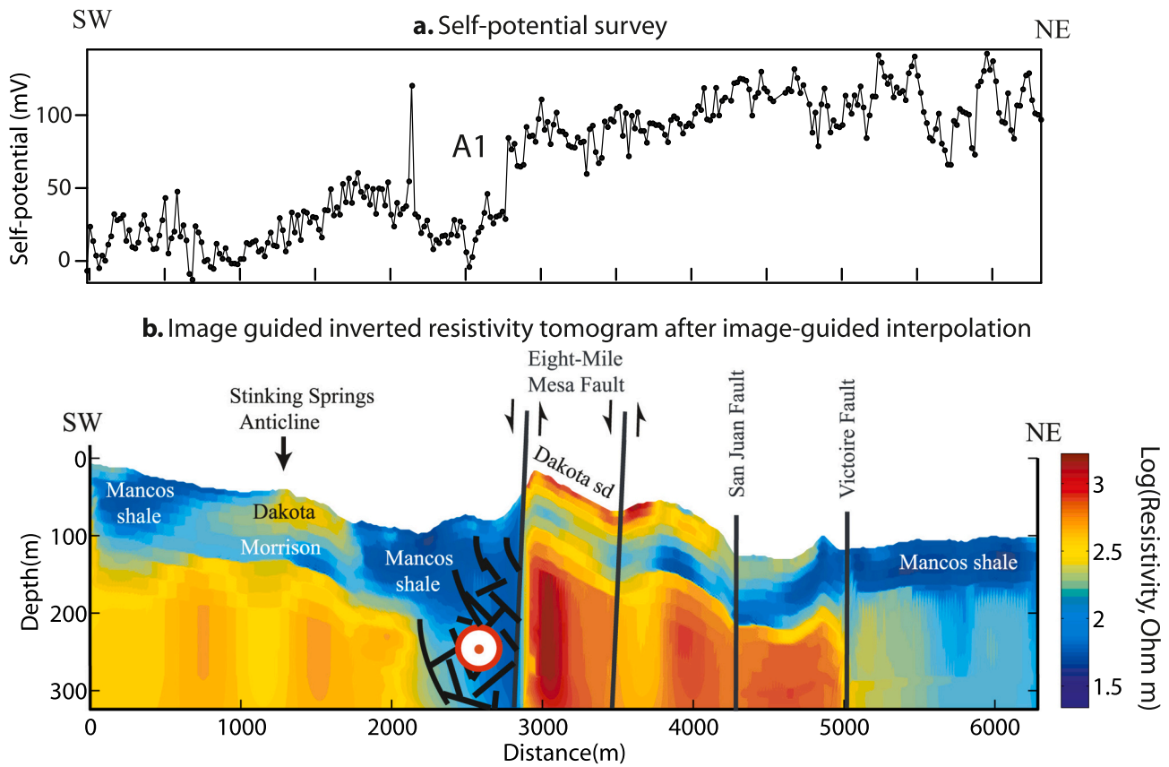
Fig. 8. The anomaly A1 (Type V) reflects the flow of hot water in the fractured hanging wall of the Eight-Mile Mesa fault (Colorado). a. Self-potential anomaly. b. Resistivity tomography (using an image-guided inversion) with the hydrogeological interpretation in terms of groundwater flow. The red arrow indicates flow normal to the plane of the section. (For interpretation of the references to colour in this figure legend, the reader is referred to the web version of this article.)
