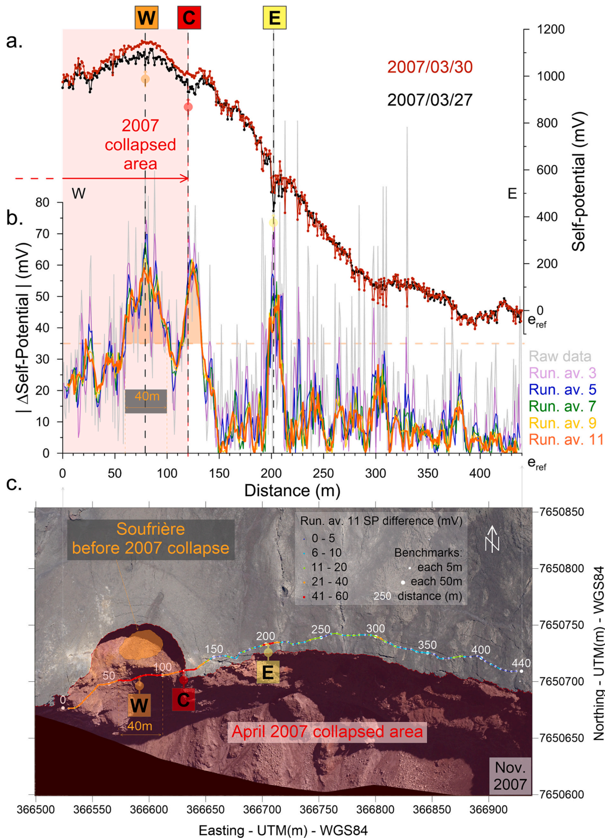
Fig. 28. Piton de la Fournaise volcano. a. Self-potential signal recorded along the profile, on March 27th and 30th 2007. b. Difference of self-potential between the two reiterations. Representation of the raw and filtered data using running averages over 3, 5, 7, 9, and 11 points. c. Aerial photograph of the studied area taken in November 2007 showing the collapsed area, the pre-collapse Soufrière pit crater, and the spatial distribution of SP anomalies along the profile. W, C, and E stand for western, central and eastern anomalies respectively (modified from Chaput et al., 2019).
