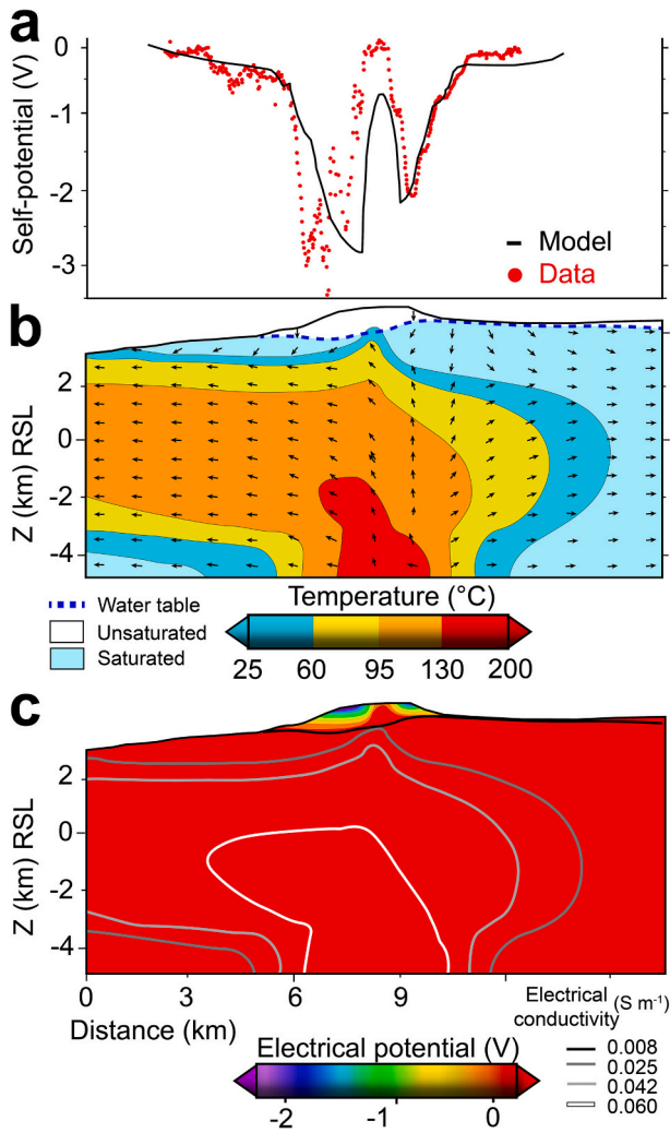
Fig. 14. Self-potential model of Ticsani volcano (Peru) obtained after post-processing finite element multiphase flow model (modified from Byrdina et al., 2013). a. Modeled “W-shaped” self-potential anomaly (black solid line) compared with real self-potential measurements (red points). b. 2-D axisymmetric fluid flow model of the volcanic island. A deep heat source is imposed at depth in the central zone, and is connected to the surface through a permeable conduit. Meteoric recharge is set at 150 mm per year, except above the central conduit region. After 30,000 years of constant heat, the thermal structure shows a hydrothermal plume (~50–200 °C) developed in the vicinity of the vertical conduit. Black arrows indicate fluid circulation, and blue dotted line represents the water table. c. Electrical potential distribution calculated from the post-processing of the multiphase flow results and its inferred conductivity structure (white-black lines). The two lobes of negative electrical potentials visible on the volcano flank (–2 V) are induced by meteoric infiltration while the central positive amplitude (+2 V) results from a combination of fluid upwelling and conductive rocks. (For interpretation of the references to colour in this figure legend, the reader is referred to the web version of this article.)
