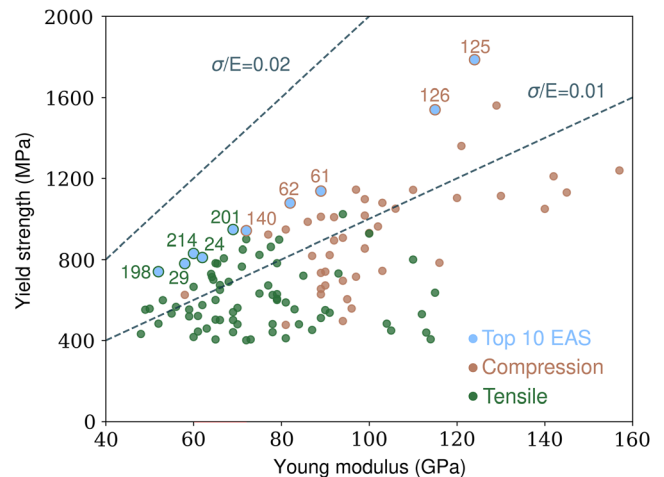
Figure 3. Reconstructed YS versus young modulus map based on dax-ti. Auxiliary design guidelines are presented as blue dashed lines. Some outstanding alloys with elevated EAS are highlighted in light blue and identified with their respective numbers from the dataset. For more information, please check Table 3.
