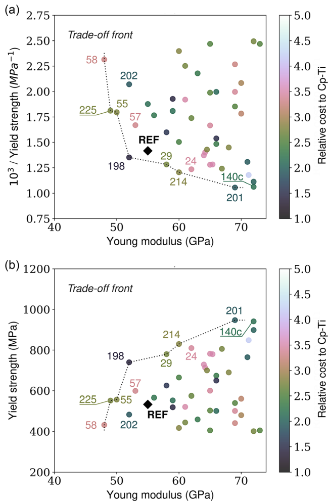
Figure 4. Trade-off frontier to aid MOOs of Ti alloys: YS versus young modulus. The higher the strength and the lower the modulus, the better. Each alloy is depicted by a color representing the alloy's relative cost relative to commercially pure Ti. The reference at the center is the benchmark alloy, TNZT (530 MPa, 55 GPa, min. of 20% deformation at the rupture) Image a) depicts the y-axis as 1/Y_S (inverted), while image b) shows the direct relationship (from lower to higher YS). Sample 140c is the only specimen depicted near the trade-off surface tested under compression.
