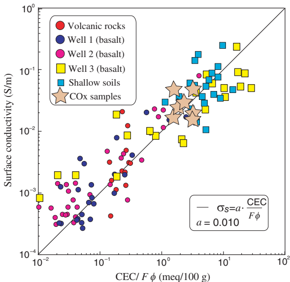
Figure 13. We use the surface conductivities from Table 1 with the formation factor determined from Archie's law with m = 2.5 and the surface conductivity data determined from the measured normalized chargeabilities.
